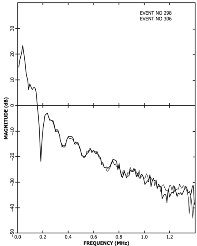
FIG. 7 Magnitude Responses of an AE Transducer as Determined by Two Calibrations with Remounting of the Transducer In Between
