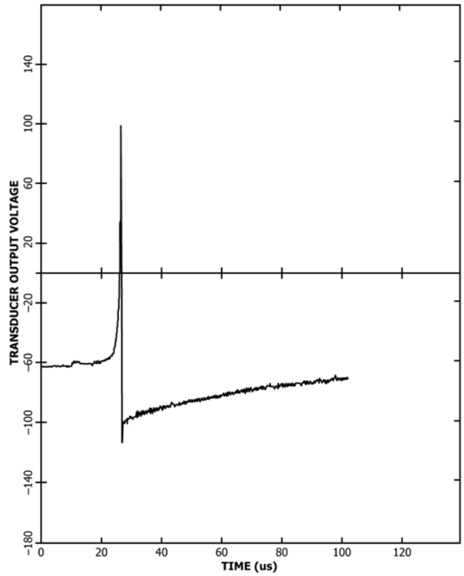
FIG. 9 A Typical Calibration—Voltage Versus Time Waveform from the Standard Transducer as Captured by the Transient Recorder (Note that the “shelf” value for the elasticity calculation of section 5.2.1 is located just after the negative going “overshoot”)
