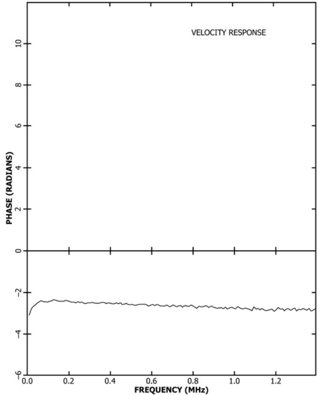
FIG. 12 Spectrum Phase Corresponding to the Spectrum Magnitude of Fig. 11
