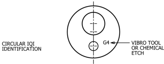
FIG. 3 Circular IQI Identification
