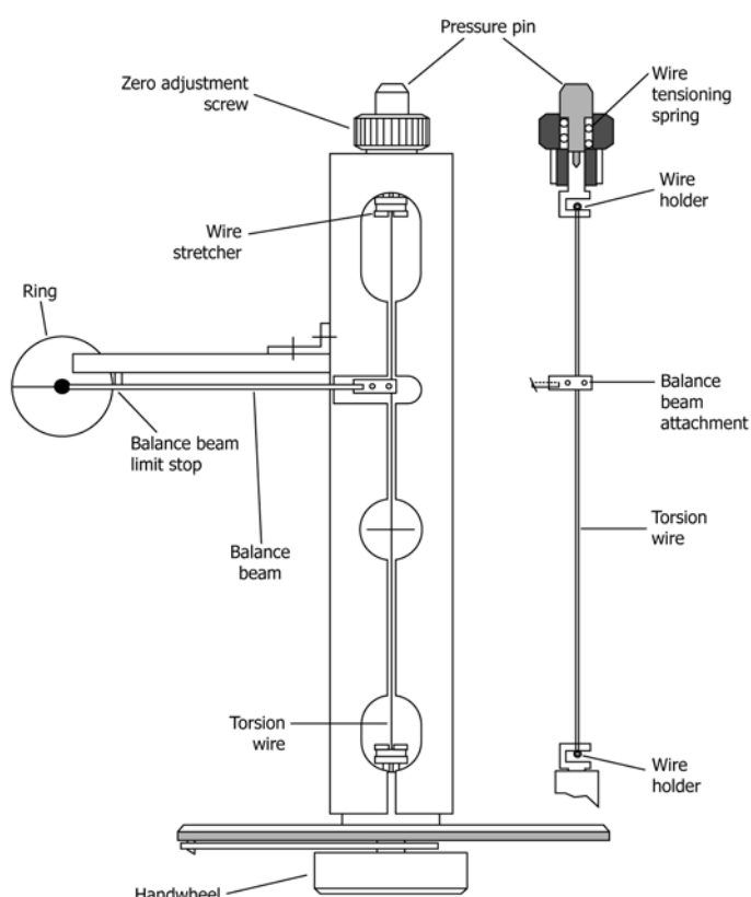
FIG. 2 Top View of Interfacial Tensiometer
