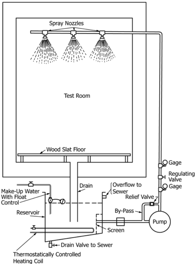
FIG. 1 Schematic Diagram of Spray Apparatus
