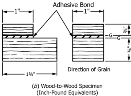
FIG. 2 Block Shear Impact Test Specimens
