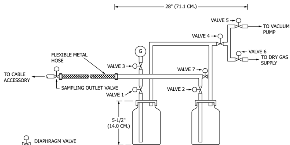
FIG. 10 Apparatus for Sampling Oil from Low-Pressure Filled Cable with Use of Vacuum and Dry Gas
