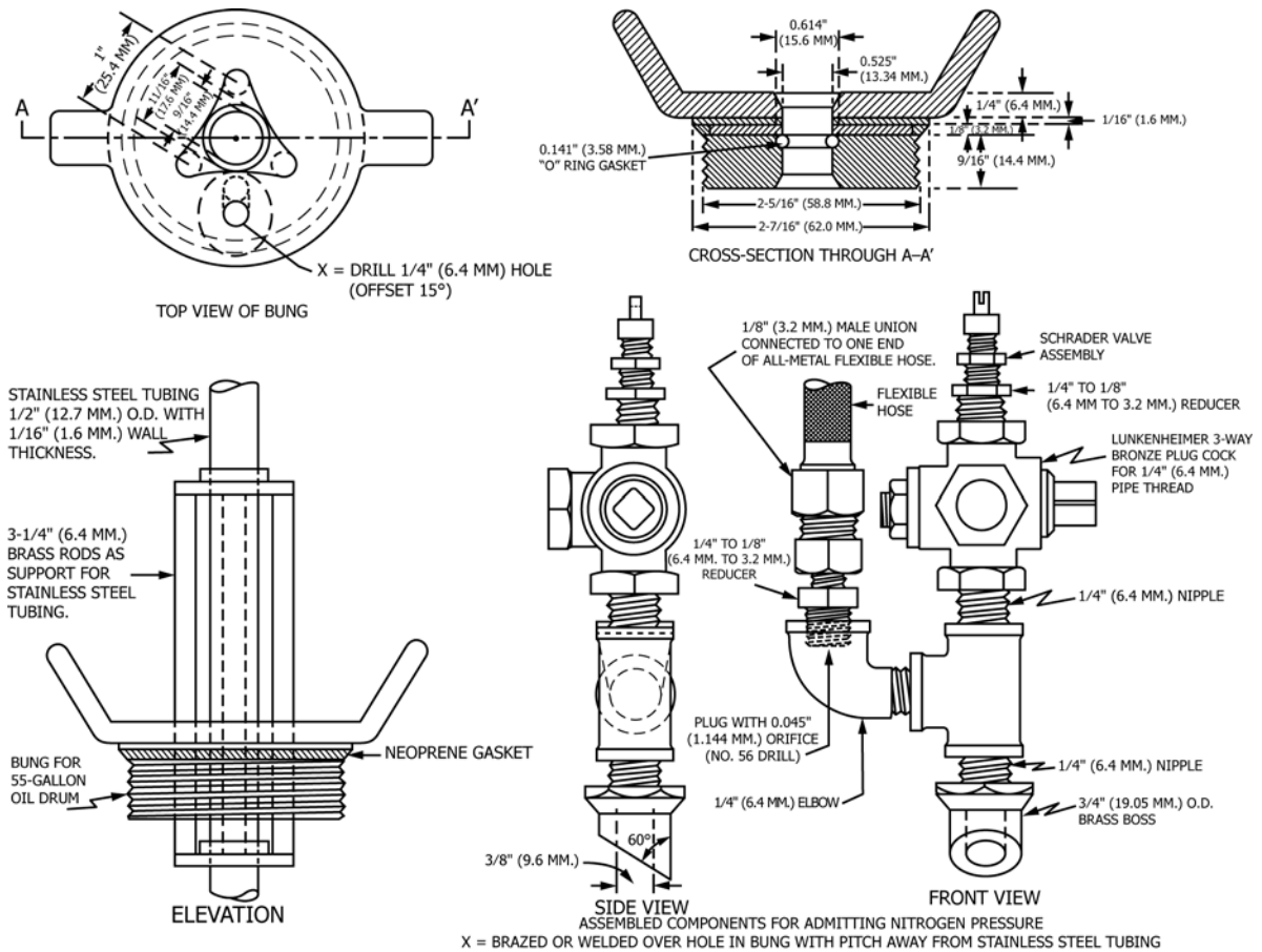
FIG. 8 Details of Bung and Fittings for Pressure-Type Sampling Devices
