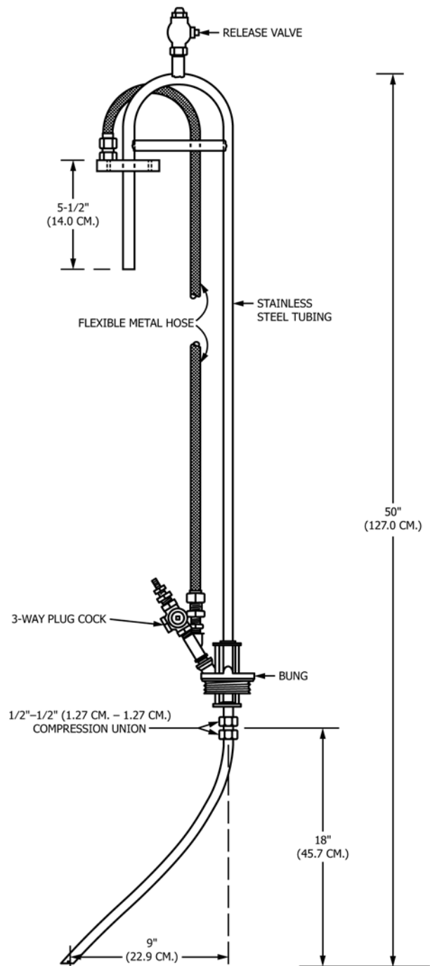
FIG. 7 Pressure-Type Sampling Device
