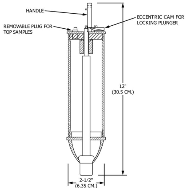
FIG. 9 Tank Car-Type Sampling Device
