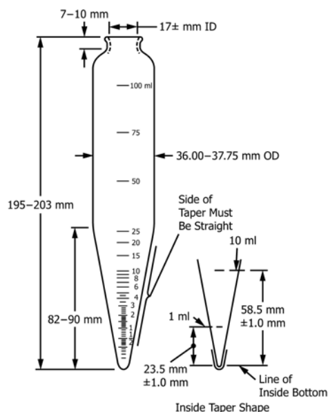
FIG. 1 ASTM Cone-Shaped Centrifuge Tube
