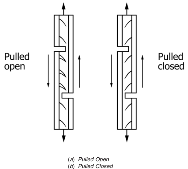
FIG. 3 Lathe and Notch Orientations for Testing
