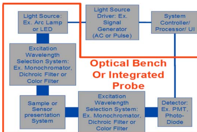
FIG. 1 Optical Bench or Integrated Probe
