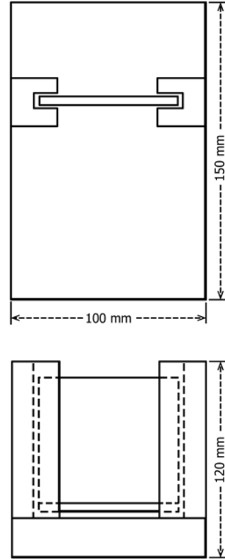
FIG. 3 Static-Mass Cement Spreader
