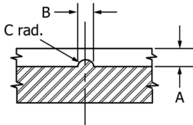
FIG. 2 Test Specimen with Circular Groove
