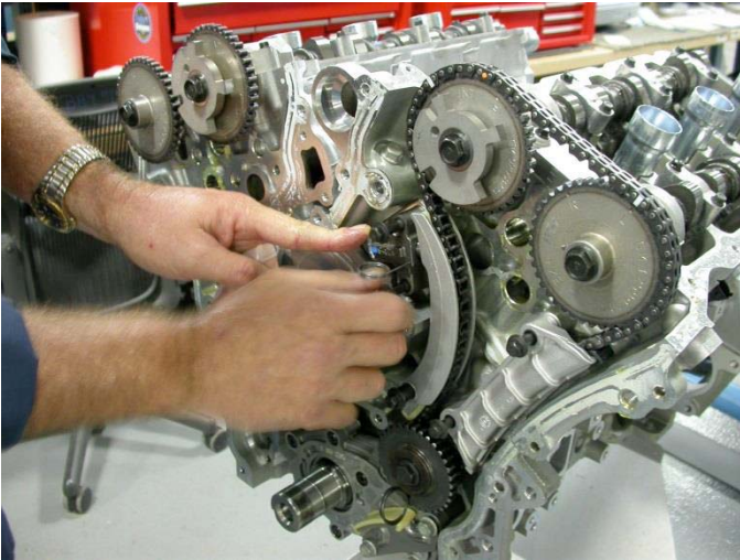
FIG. A17.5 Installation of Chain Guide, Tensioner and Gasket, Left Side
