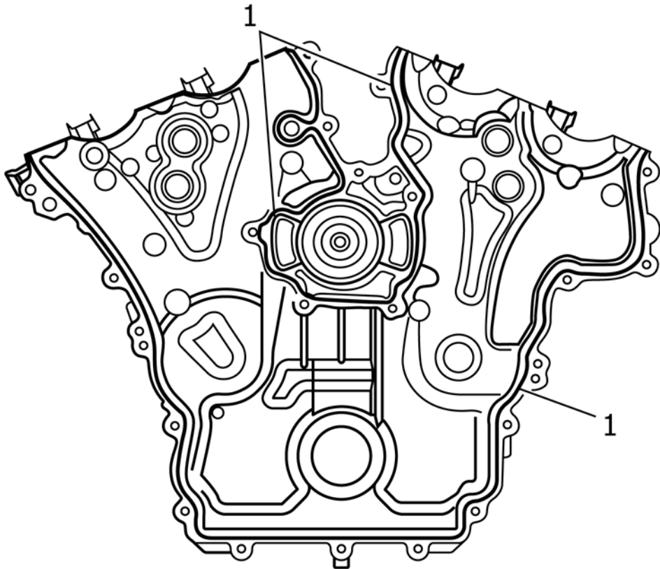
FIG. A17.18 Location of RTV Bead Placement
