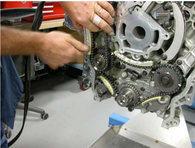
FIG. A17.12 View Showing Chain Guide and Tensioner Installation
