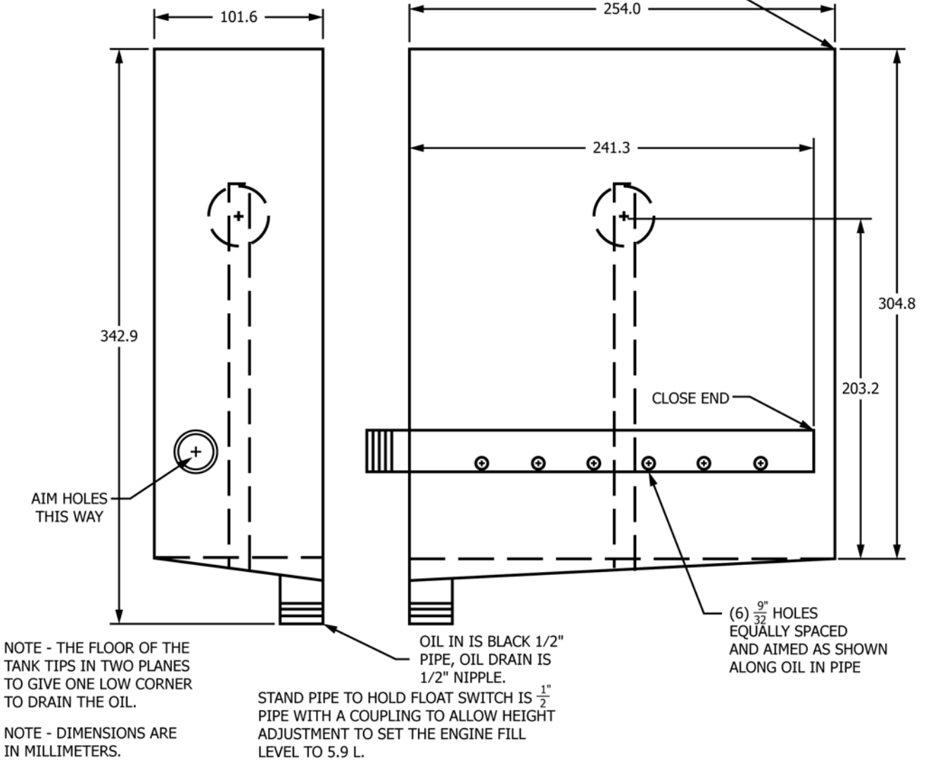
FIG. A5.8 Typical Oil Dump Tank
