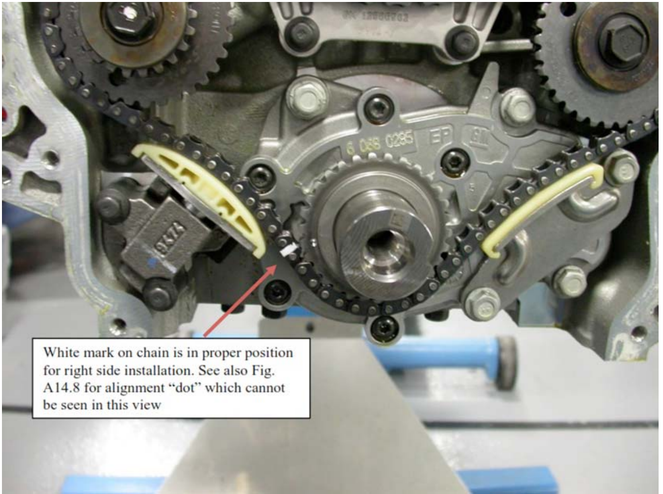
FIG. A17.10 View Showing Timing Proper Alignment
