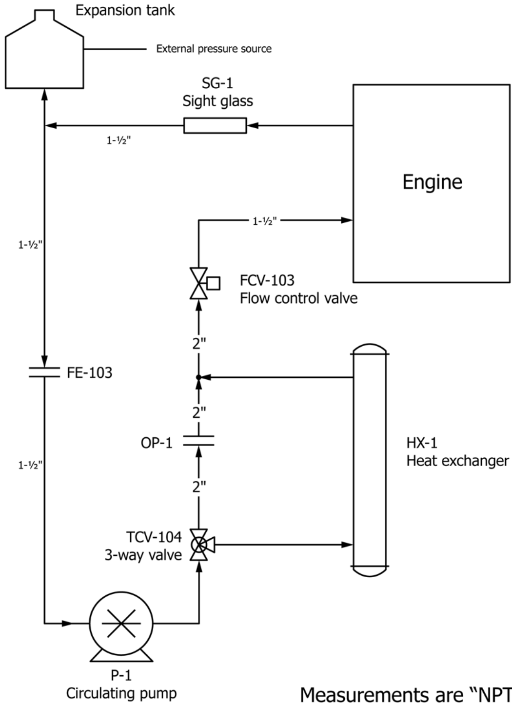
FIG. A5.1 Typical Engine Cooling System
