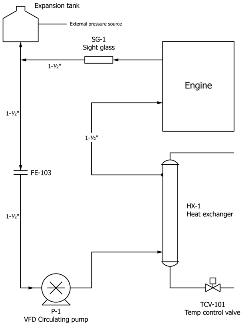
FIG. A5.3 Alternative Cooling System with VFD
