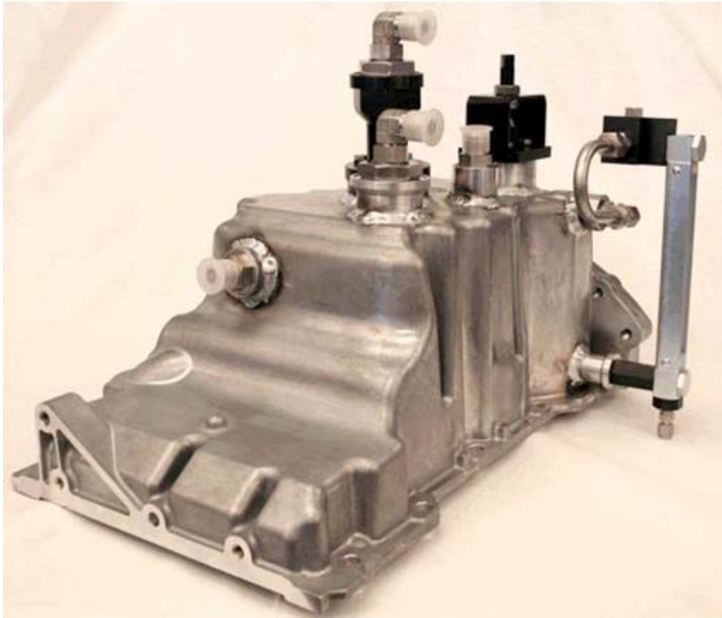
FIG. A5.9 Sequence VIE Pan Modifications
