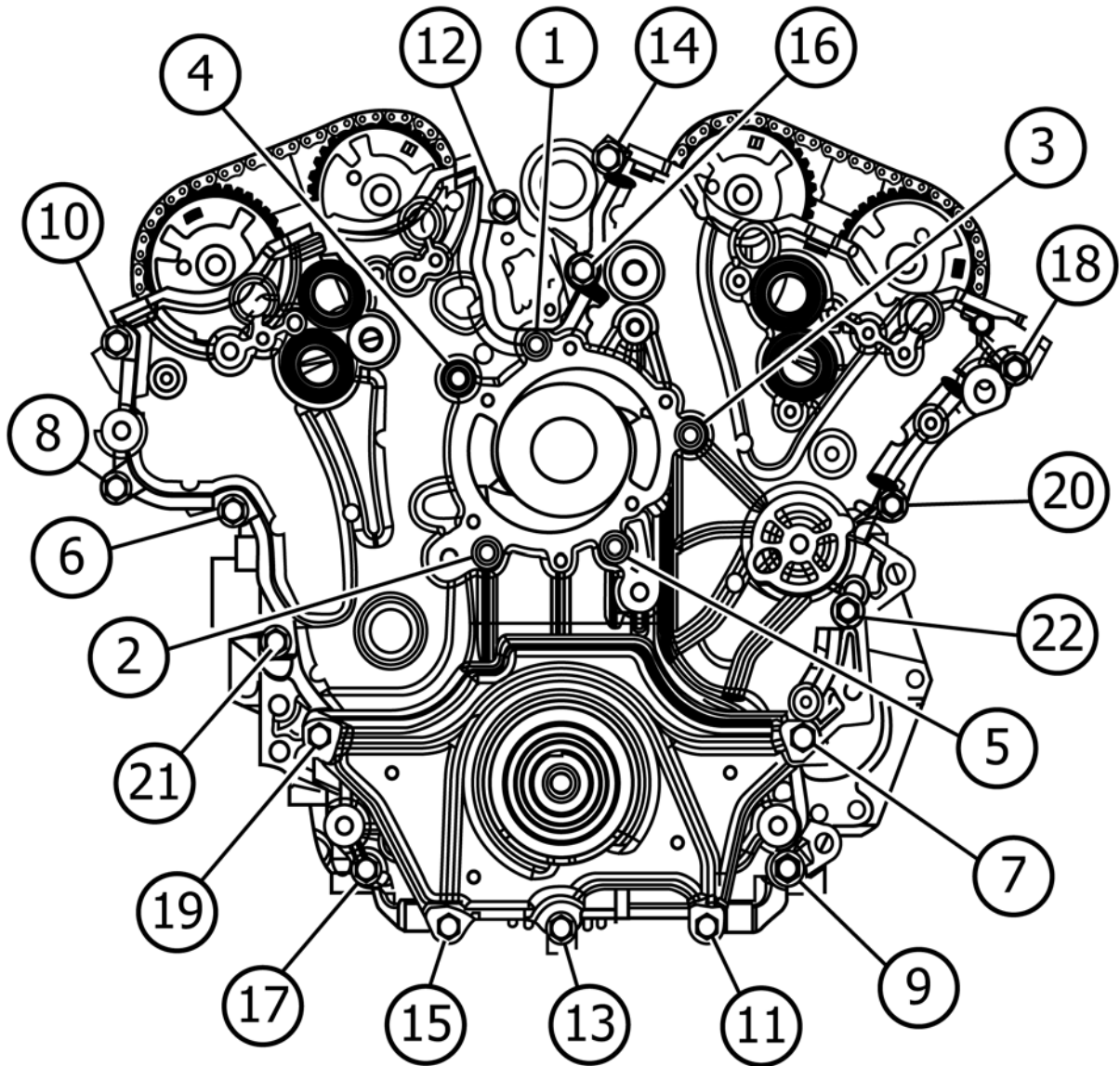
FIG. A17.21 Tightening Sequence for Front Cover
