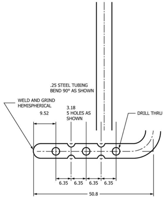
PROBE DETAIL
