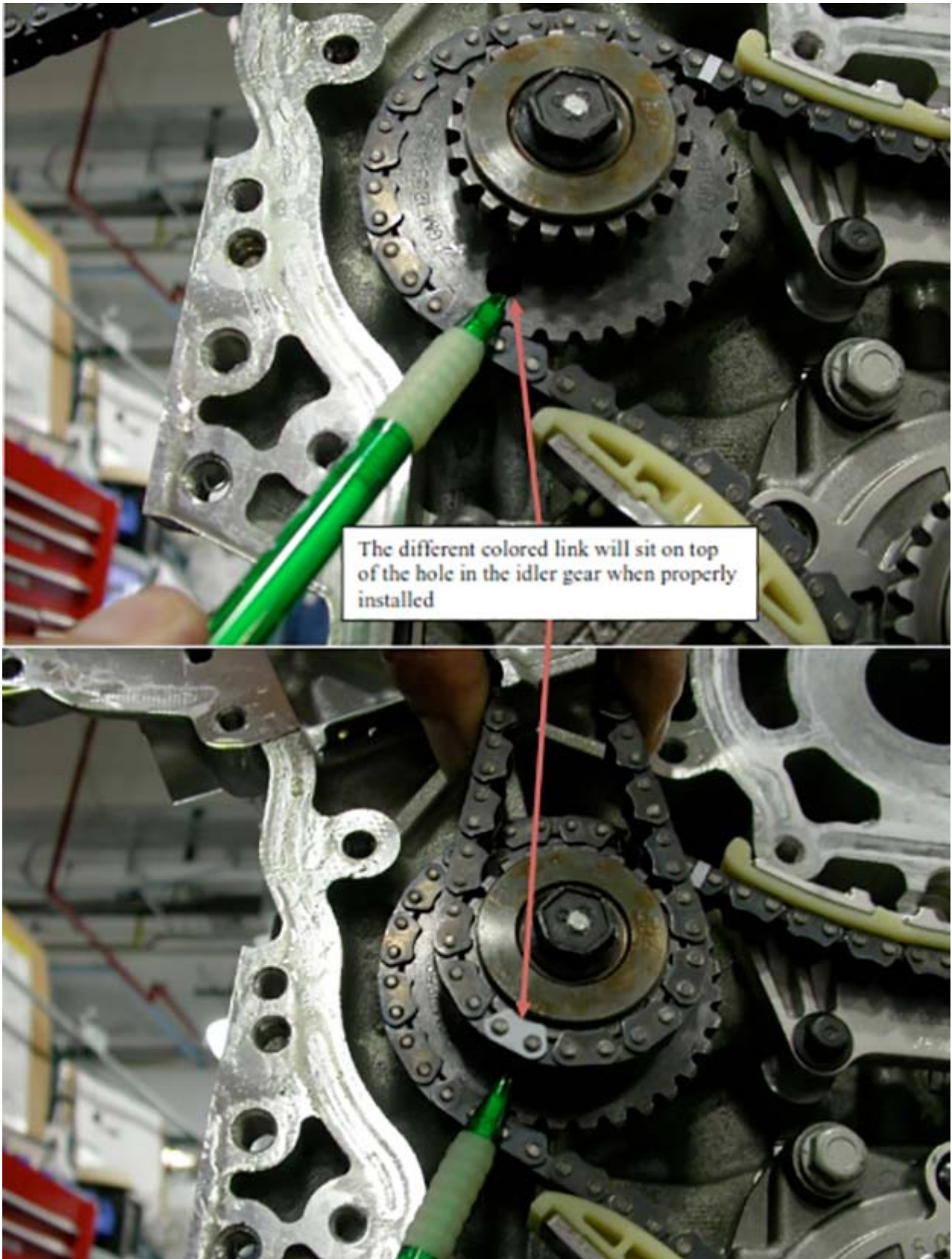
FIG. A17.11 View Showing Proper Gear Alignment for Right Side
