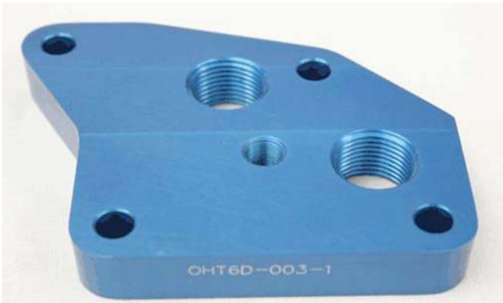
FIG. A5.10 Oil Filter Adapter Assembly
