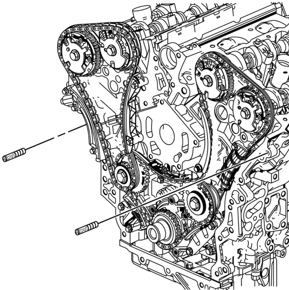
FIG. A17.16 Location of Guide Pins
