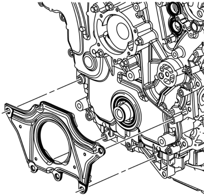
FIG. A17.20 Front Cover Sound Deadener Installation
