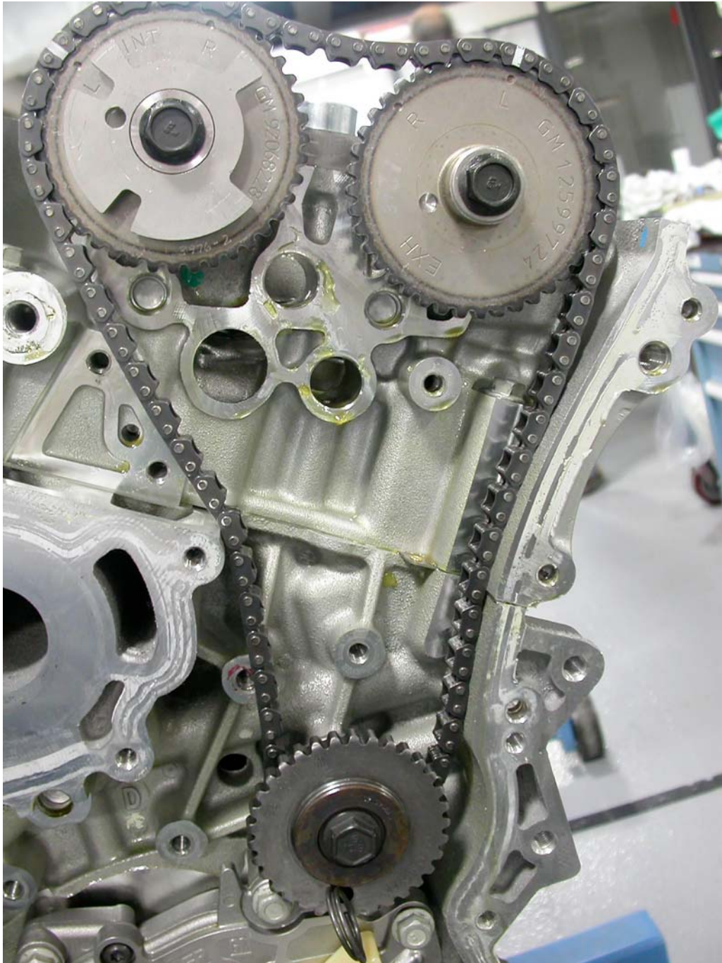
FIG. A17.4 Alignment of Timing Marks, Left Side, with Grenade Pin Installed
