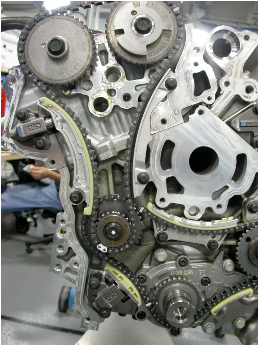
FIG. A17.15 Right Side Chain and Idler Alignment Marks
