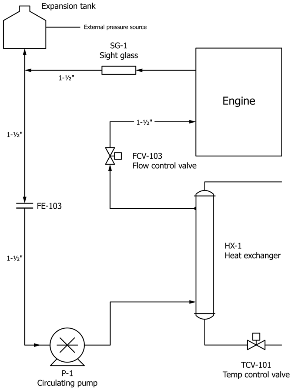
FIG. A5.2 Alternate Cooling System
