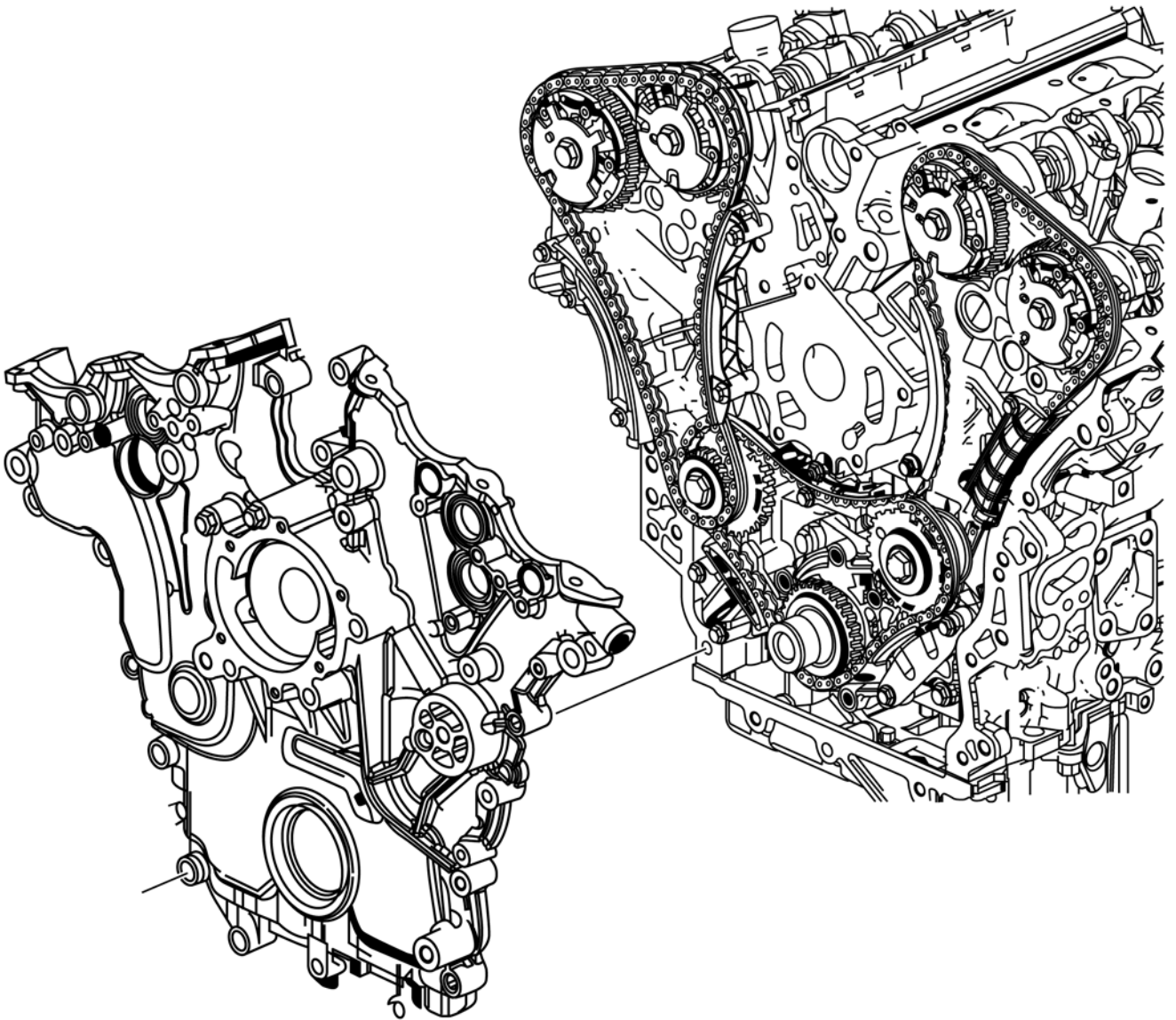
FIG. A17.19 Installation of Front Cover
