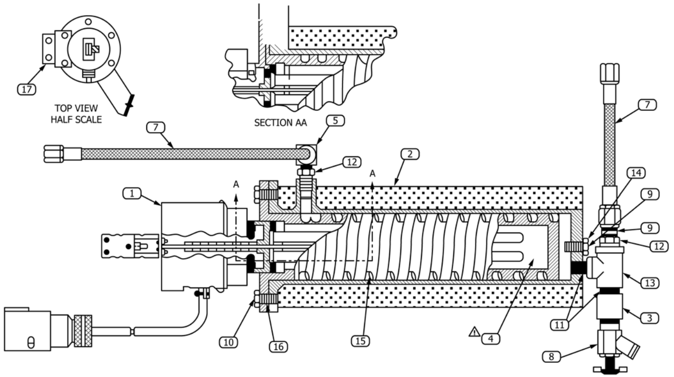
FIG. A5.7 Thermocouple in Oil Heater
