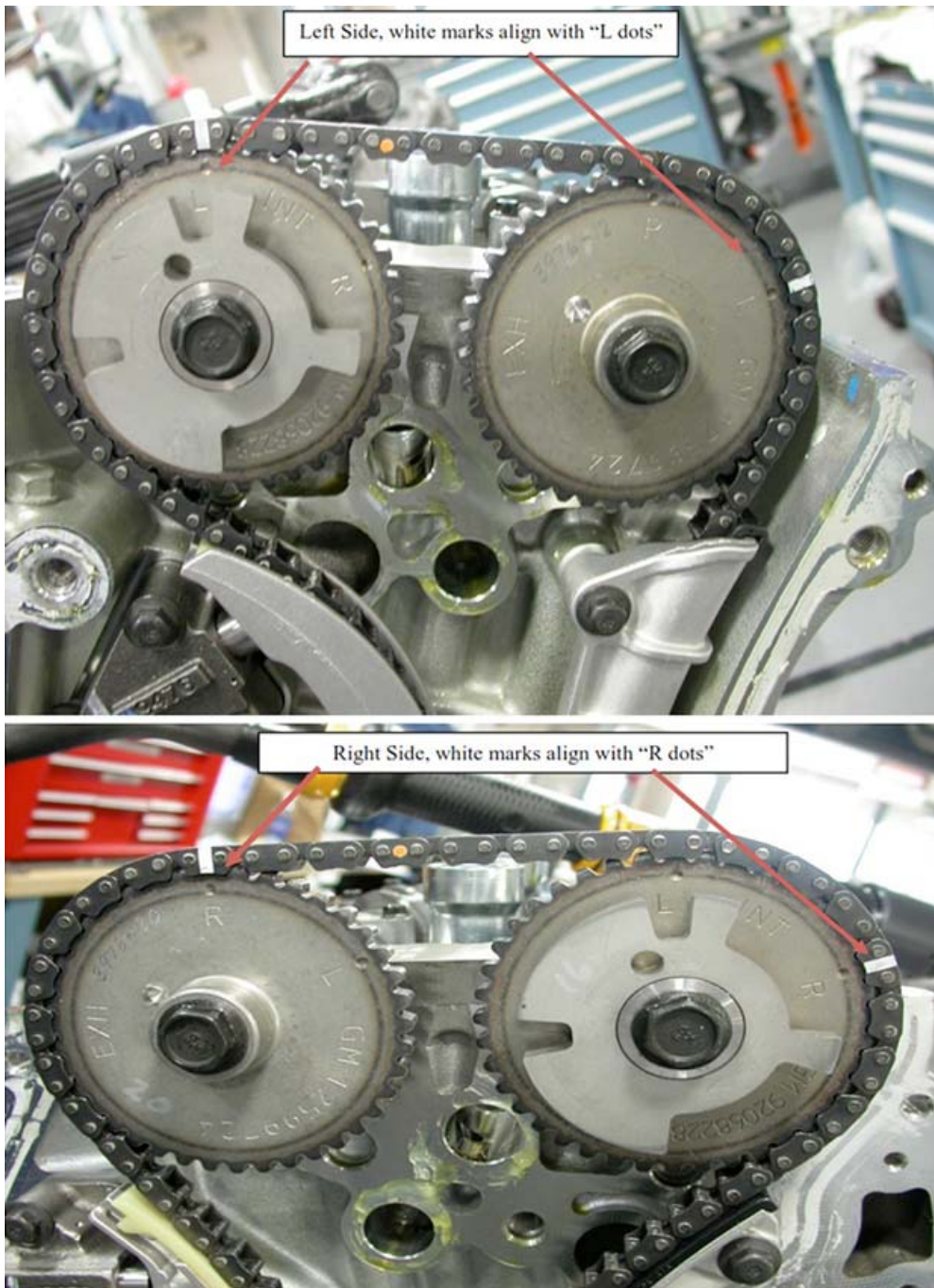
FIG. A17.14 Views Showing Proper Alignment, Left and Right Chains
