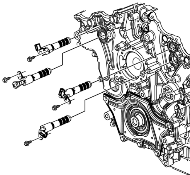
FIG. A17.22 Cam Position Actuator Location
