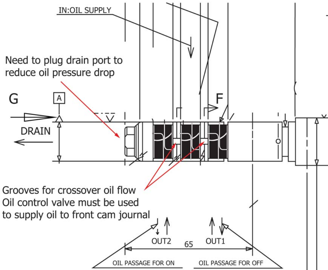
FIG. A5.21 Camshaft Position Actuator Modifications
