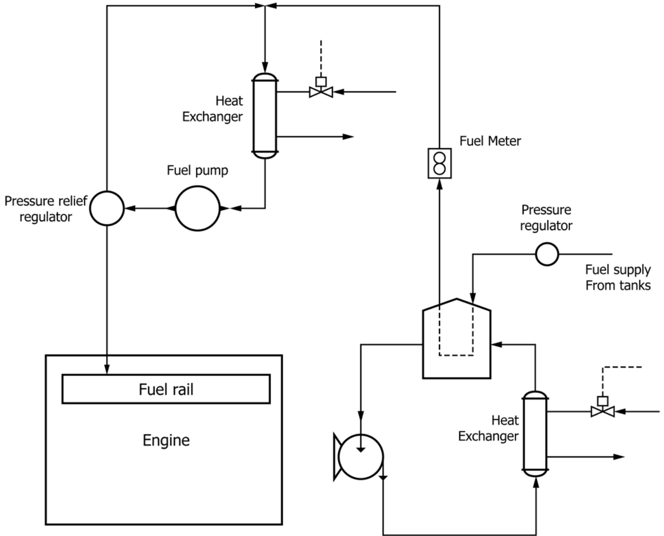
FIG. A5.11 Typical Fuel Delivery System
