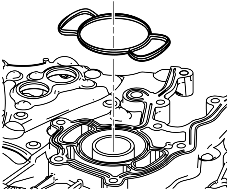
FIG. A17.17 Location of Front Cover Seal
