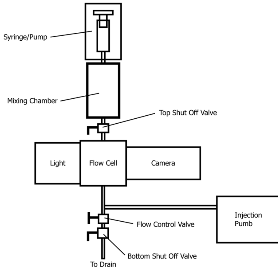
FIG. A1.1 Instrument with Injection Pump for Dilution and Syringe Pump to Meter in Specimen
