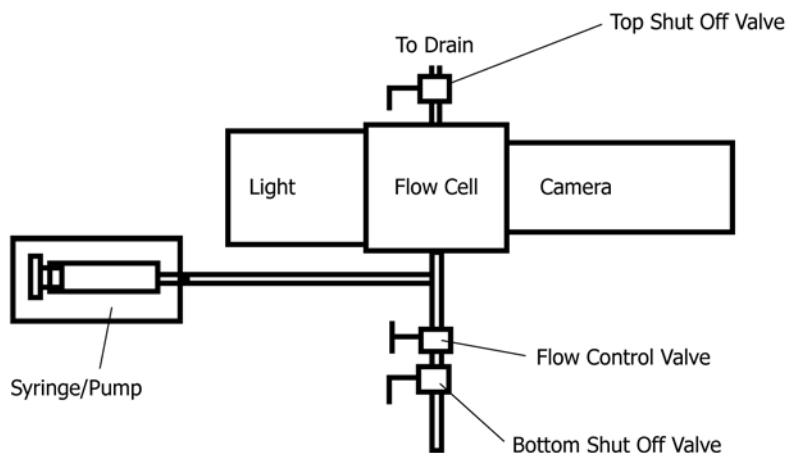
FIG. A1.2 Second Automated Configuration
