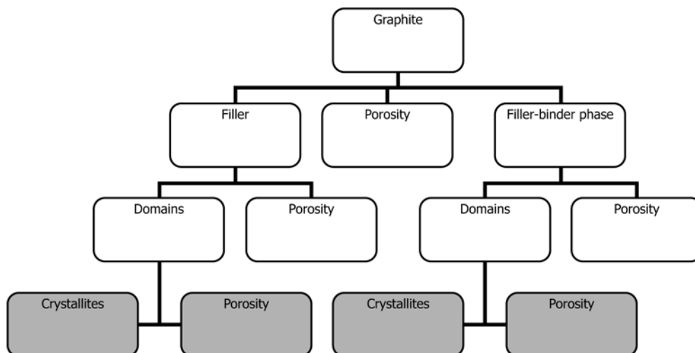
FIG. 4 Schematic Showing Hierarchy of Principal Microstructural Terms for Graphite on the Optical Scale
