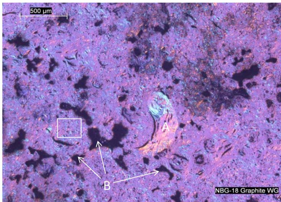
(A) Highly oriented segment of a filler coke particle (the color changes indicating changing orientation); (B) Porosity and a mosaic cluster (boxed area).
