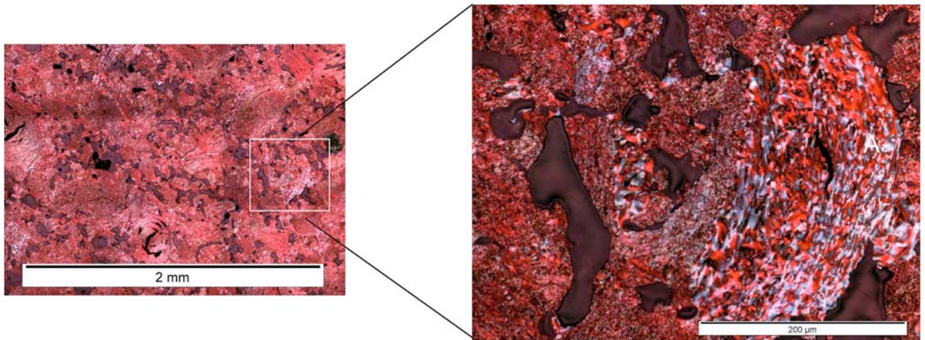
FIG. 10 Optical Micrograph Showing Mosaic Ribbon (Within Box on Left-Hand Image) and Detail of Feature (Right-Hand Image) Under Polarized Light (Gilsocarbon Graphite)
