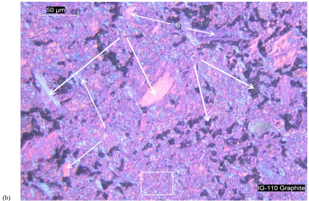
(a) Lower magnification and (b) higher magnification, showing (A) highly oriented and (B) small filler particles, and (C) porosity and mosaic texture in the filler-binder phase (boxed area).
