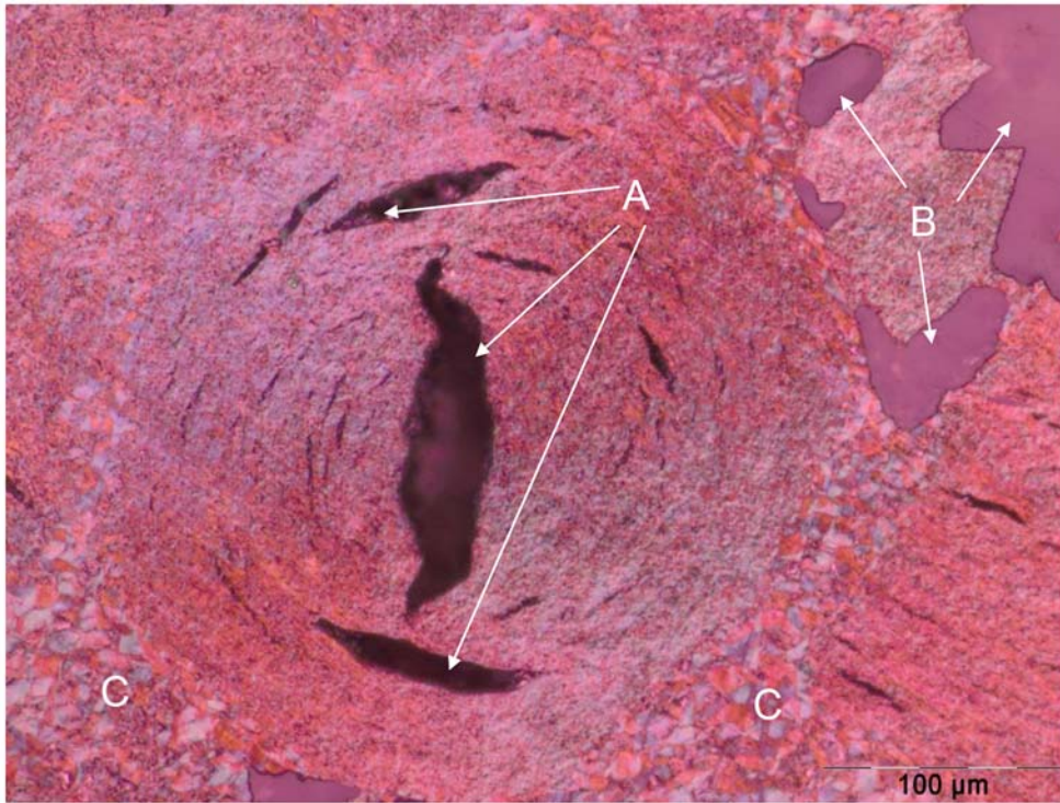
FIG. 9 Optical Micrograph Showing Mosaic Ribbons (C) at a Filler Particle Boundary Under Polarized Light with Closed Porosity (A) and Open Porosity (B) (Gilsocarbon Graphite)
