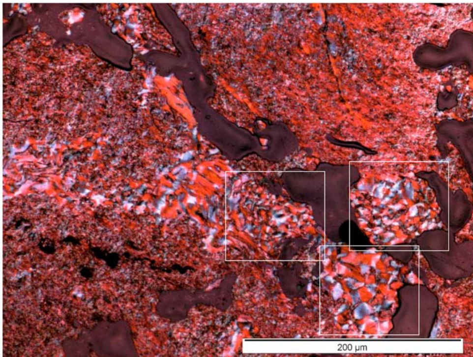
FIG. 8 Optical Micrograph Showing Mosaic Clusters (Boxed Areas) Adjacent to Closed Pores (Dark Regions) Under Polarized Light (Gilsocarbon Graphite)
