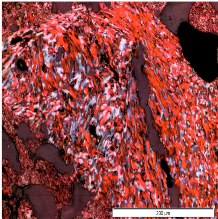
FIG. 11 Optical Micrograph Showing Supra Mosaic Under Polarized Light (Gilsocarbon Graphite)
