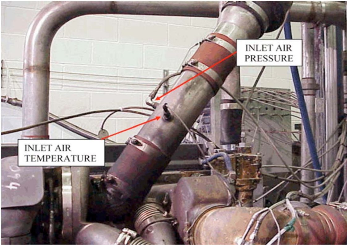
FIG. A5.7 Inlet Tube
