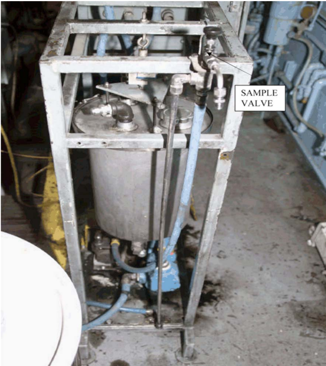
FIG. A5.10 Oil Mass Cart
