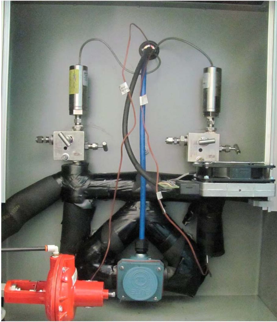
FIG. A7.2 Aeration Measurement System and Enclosure
