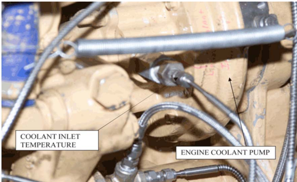
FIG. A5.14 Coolant to Engine
