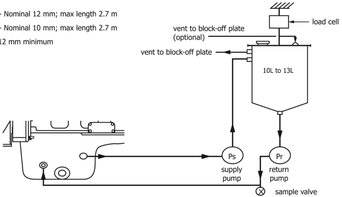
FIG. A6.1 External Oil System
