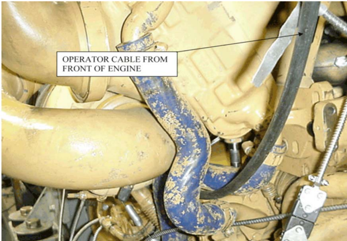
FIG. A5.22 Turbocharger Wastegate Control Cable
