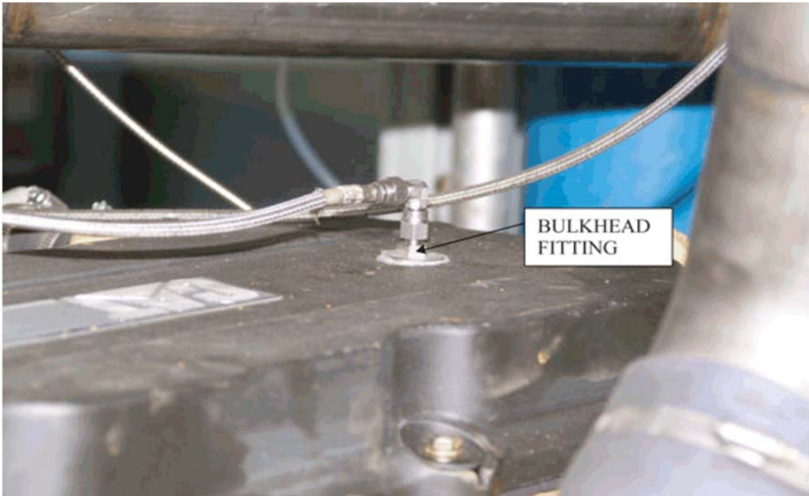
FIG. A5.12 Connection for Crankcase Pressure
