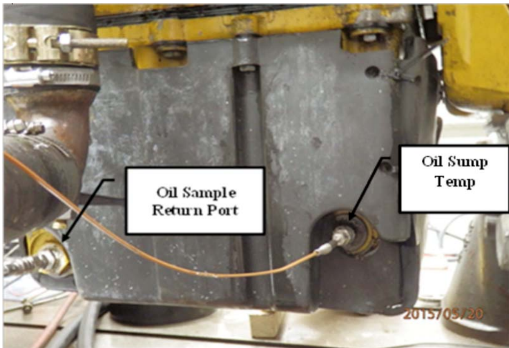
FIG. A5.5 Oil Sample Return and Oil Sump Temperature Location
