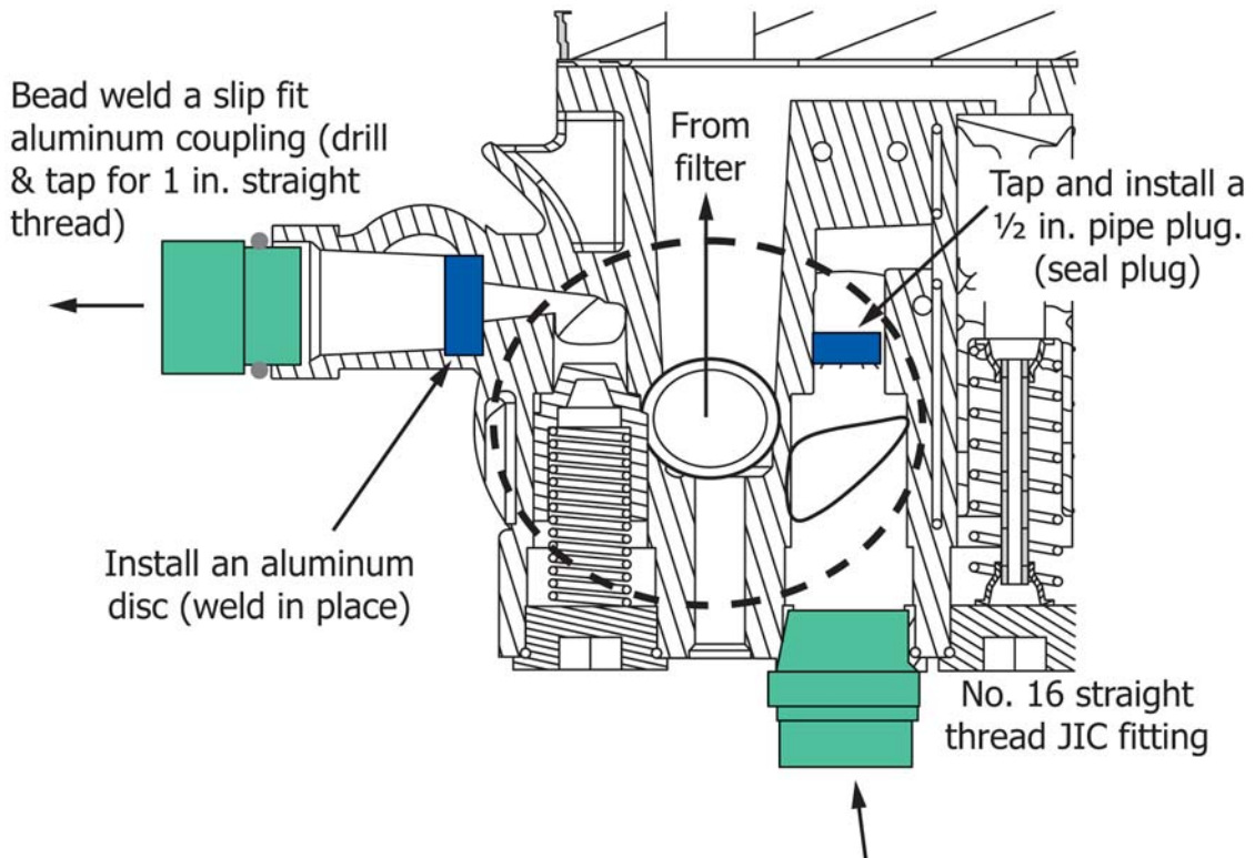
FIG. A4.3 Filter Base Modifications
