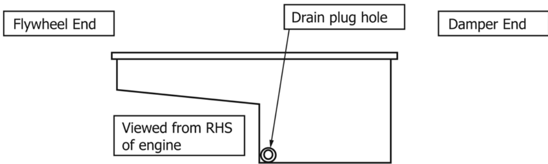
FIG. A5.4 Oil Pan Modifications for External Oil System—Auxiliary Oil System Return Port Location
