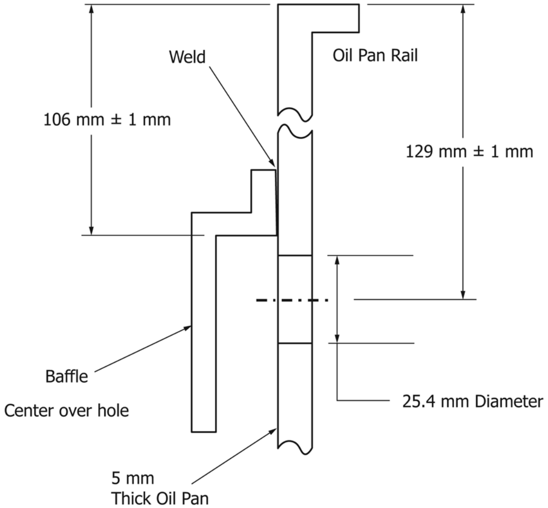
FIG. A5.3 Oil Pan Modifications for External Oil System—Baffle Placement on Oil Pan
