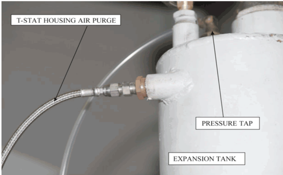
FIG. A5.18 Measurement of Cooling-System Pressure
