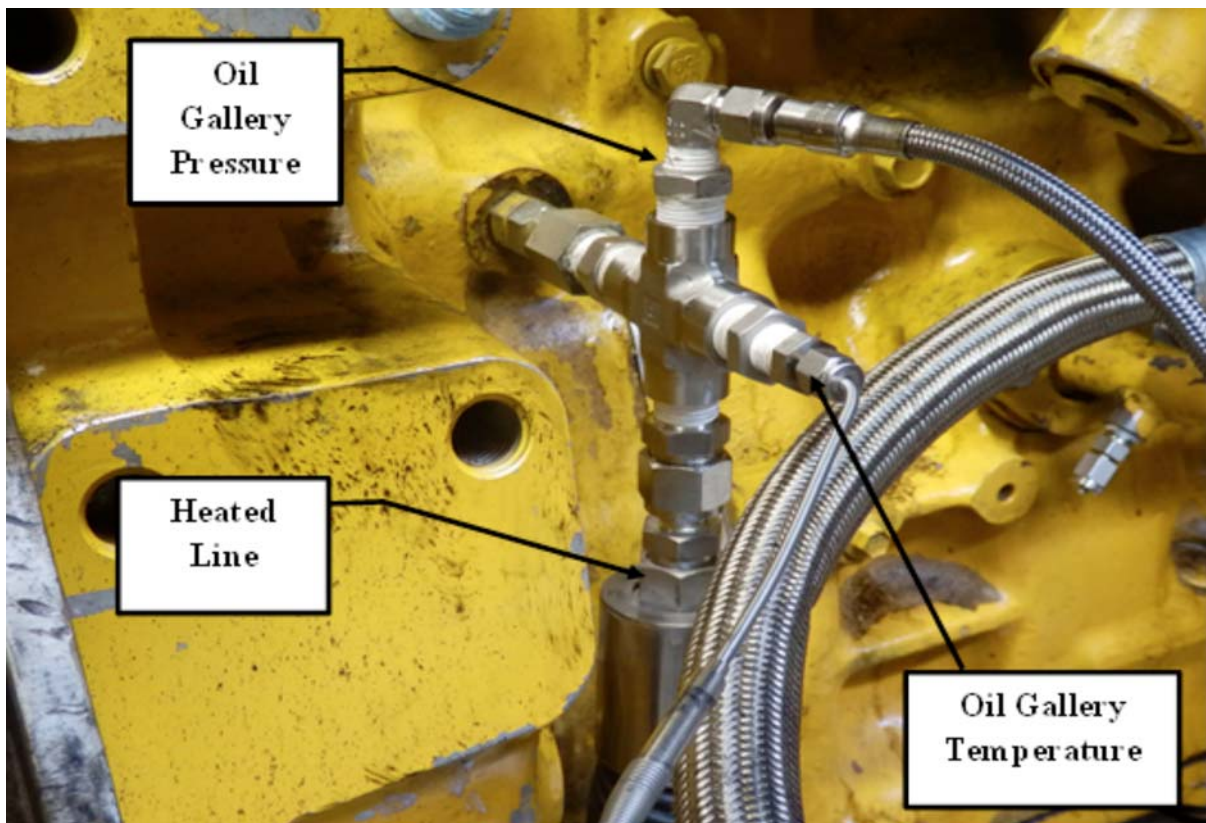
FIG. A5.15 Oil-Gallery Sample Fitting with Heated Line, Pressure and Temperature Measurements
