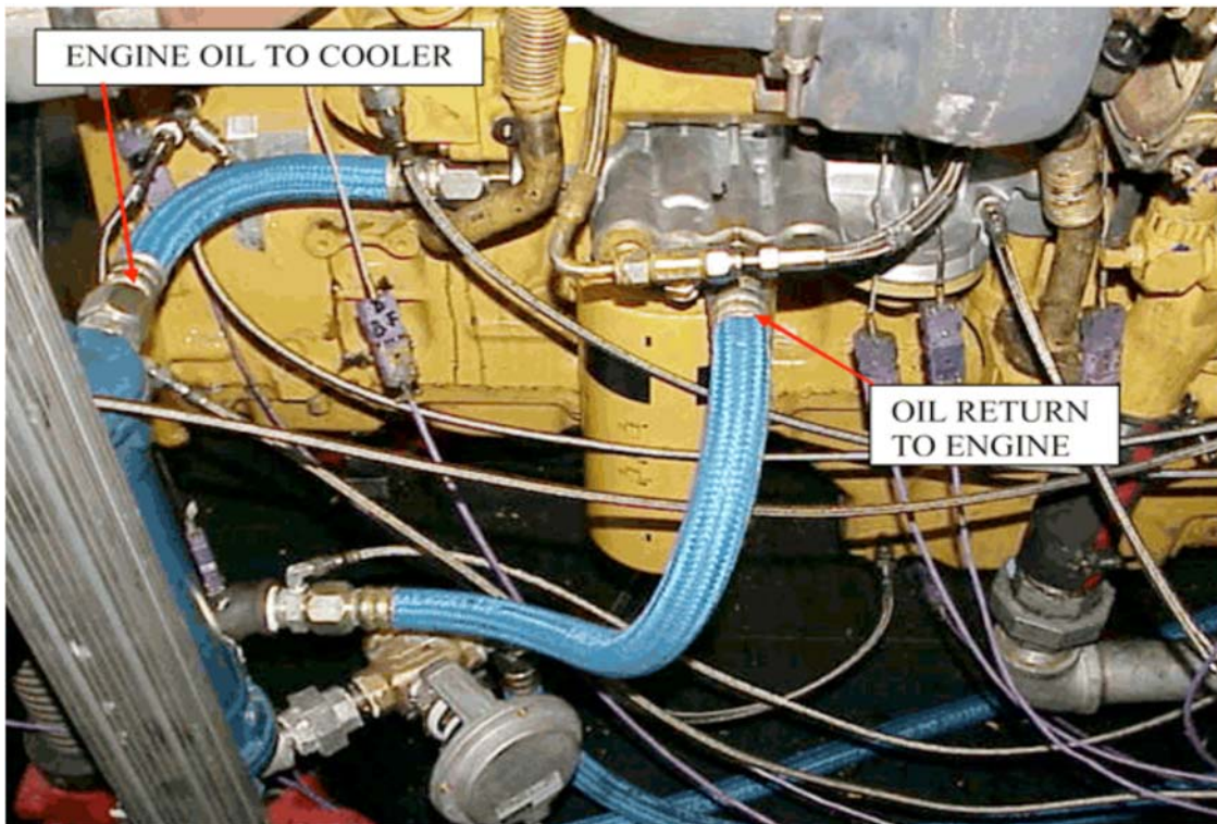
FIG. A4.1 Remote Oil Heat Exchanger
