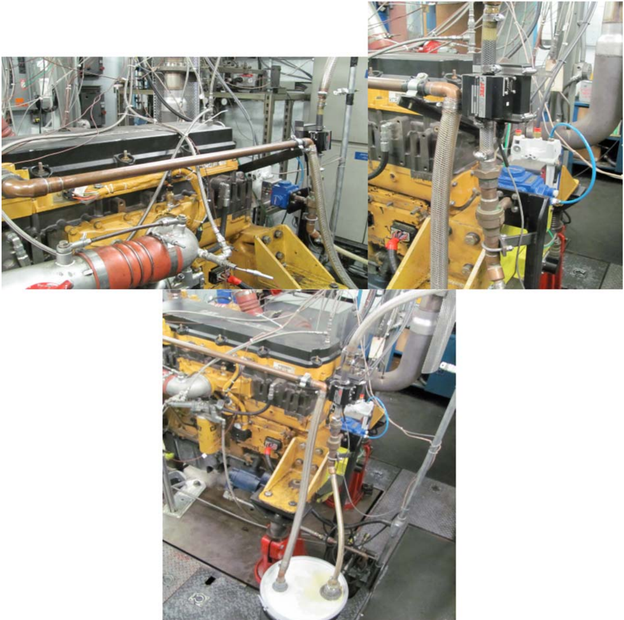
FIG. A5.11 Control System for Blowby Flow and Crankcase Pressure
