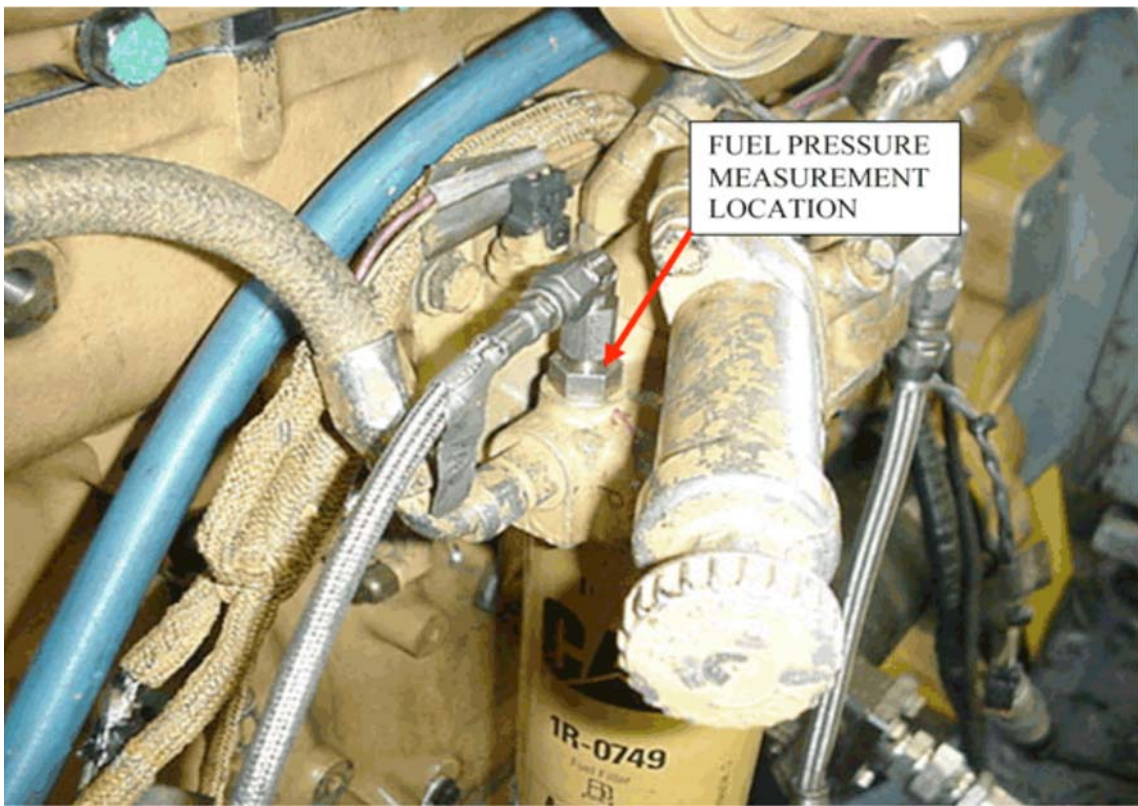
FIG. A5.25 Location of Fuel-Pressure Measurement
