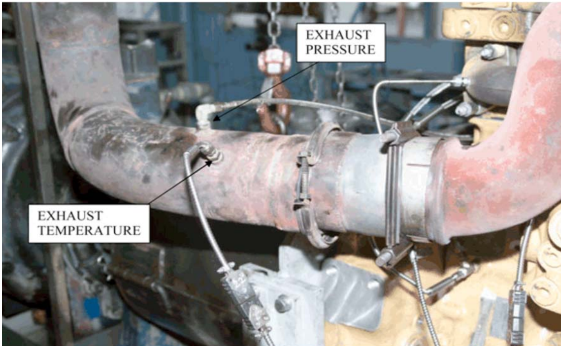
FIG. A5.8 Exhaust Tube
