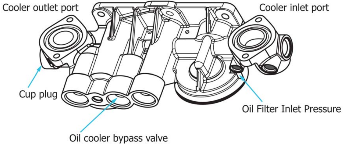
FIG. A4.2 Filter Base (P/N 251-6668) View
