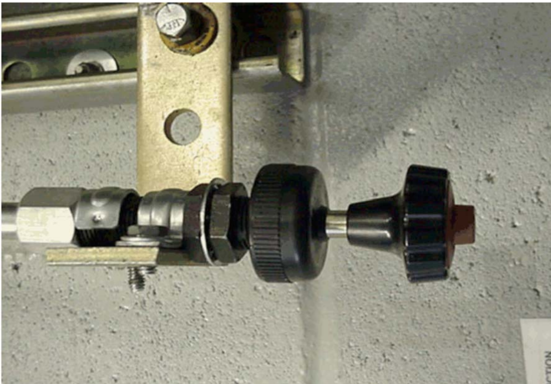
FIG. A5.23 Manual Adjuster for Turbocharger Wastegate Control
