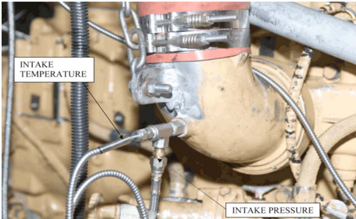
FIG. A5.17 Measurement of Intake-Manifold Pressure and Temperature
