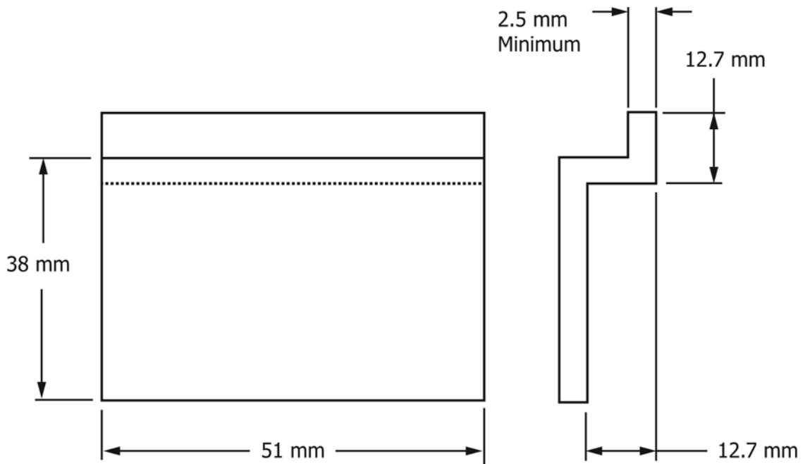
FIG. A5.2 Oil Pan Modifications for External Oil System—Suction Port Baffle Design
