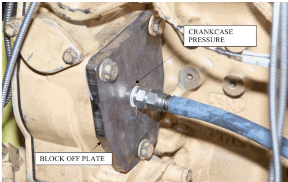
FIG. A5.6 Connection for Compressor Block-off Plate and Crankcase Pressure Balance
