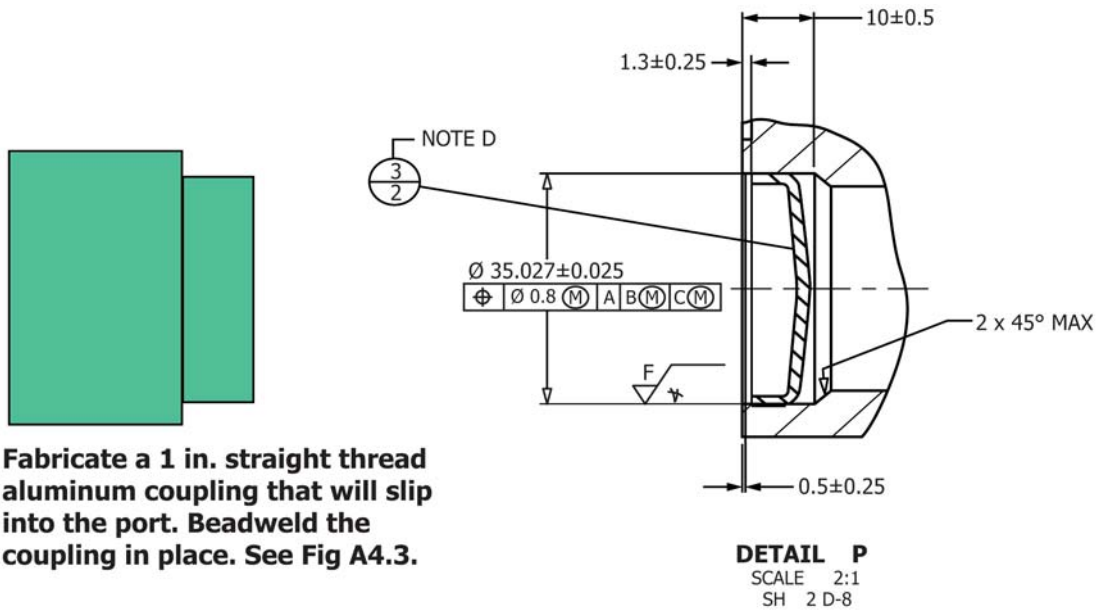
FIG. A4.4 Details of Cup Plug Feature at Back End of Filter Base
