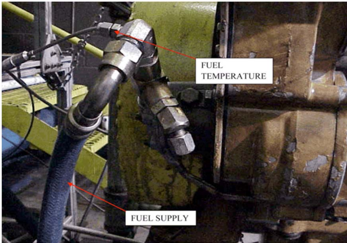
FIG. A5.16 Measurement of Fuel-to-Engine Temperature
