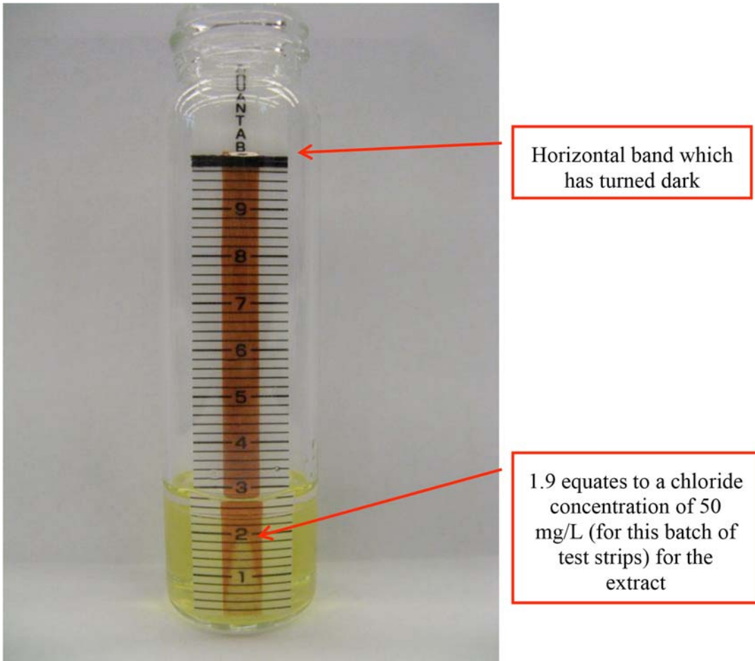
FIG. 9 Chloride Test Strip
