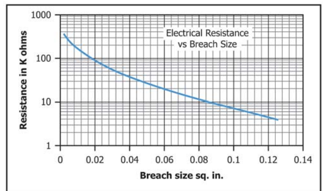
FIG. 8 Leakage Resistance Versus Membrane Breach Size
