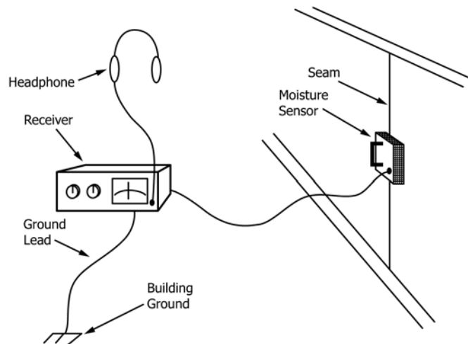
FIG. 5 Basic Circuit of Vertical Surface Leak Locate Unit
