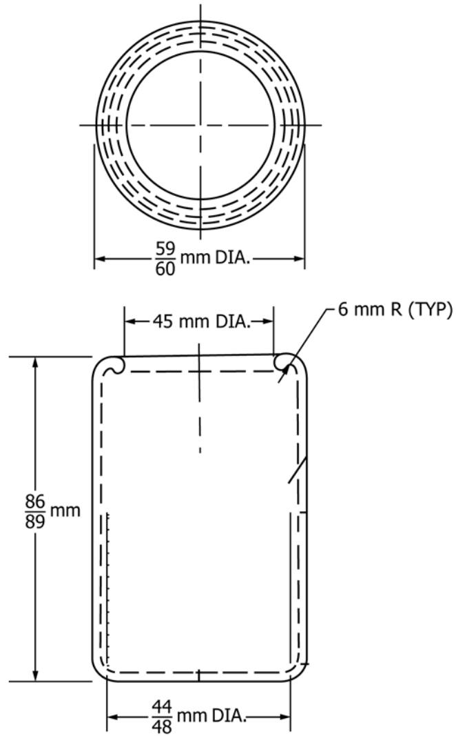
FIG. A1.3 Borosilicate Glass Sample Container
