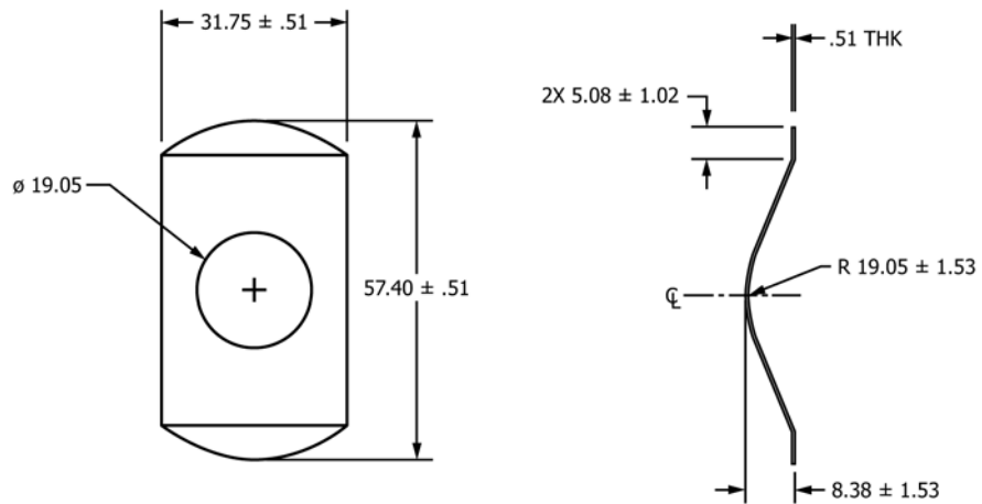
FIG. A1.4 Hold-Down Spring (bottom)
