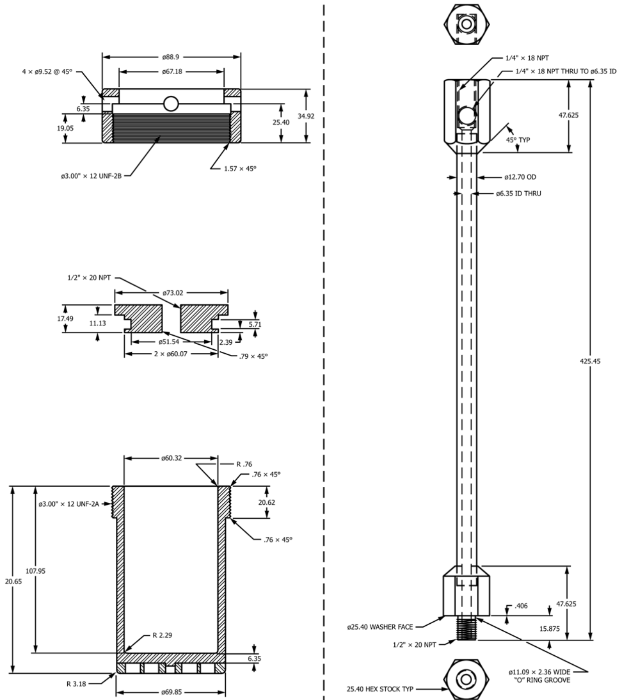
FIG. A1.2 Construction of Oxidation Vessel
