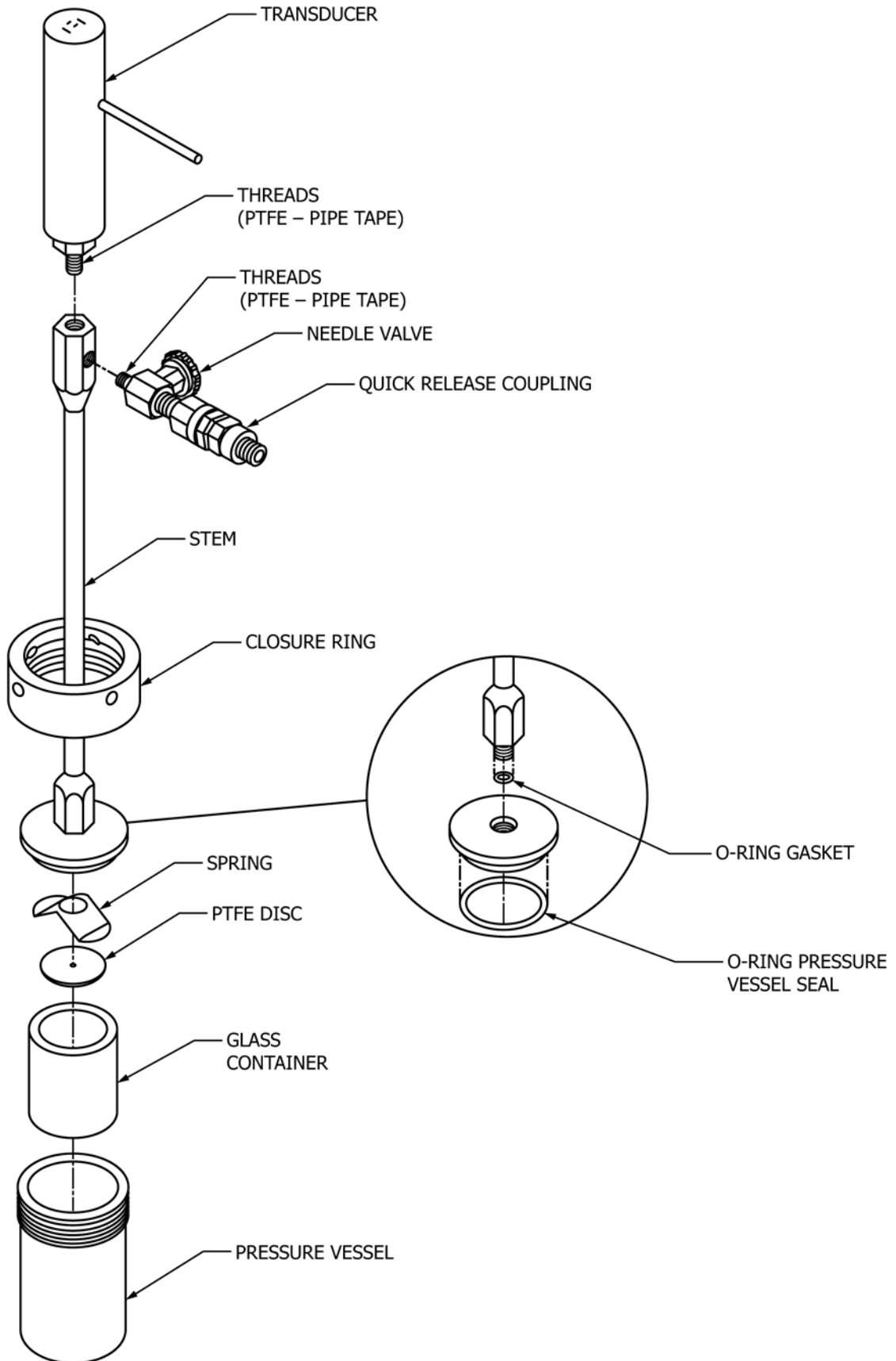
FIG. A1.5 Oxidation Vessel Assembly
