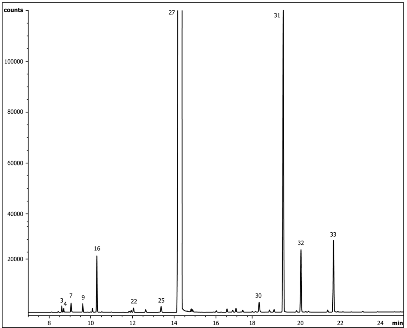
FIG. 1 Typical Chromatogram of an ETBE Sample Analyzed on a 100 Meter Column
