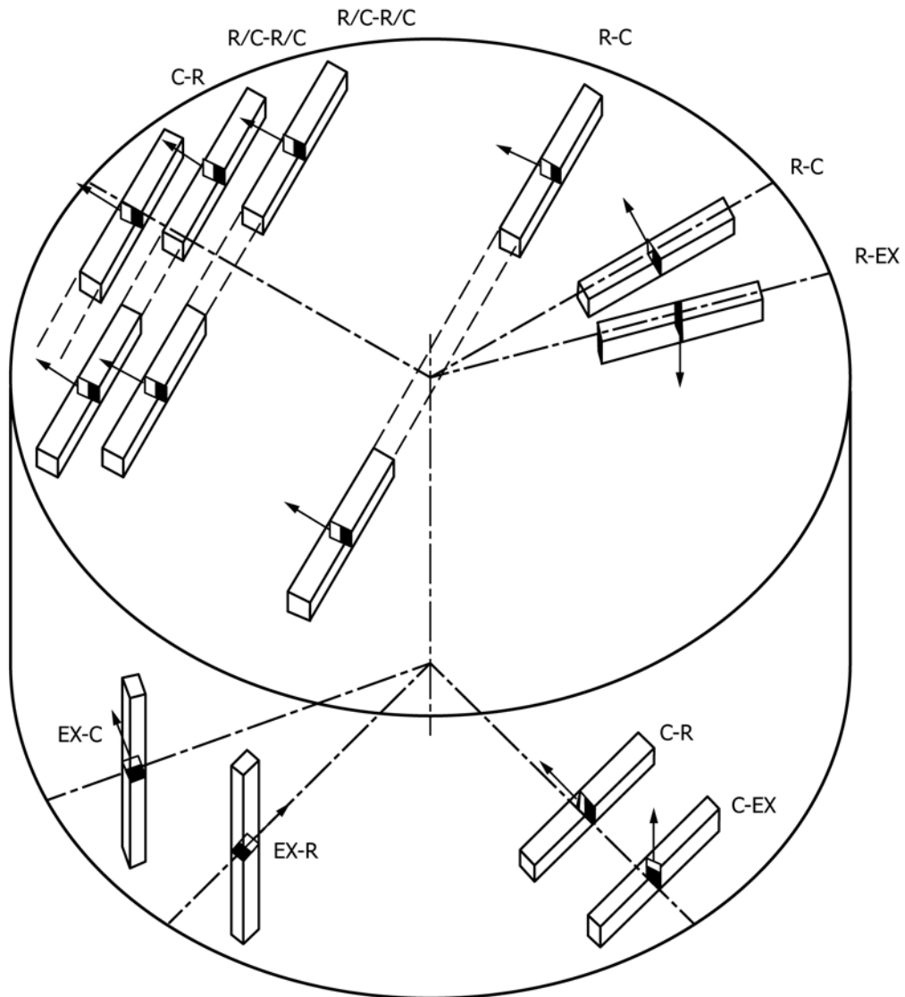
FIG. A1.1 Crack-Plane Orientation
