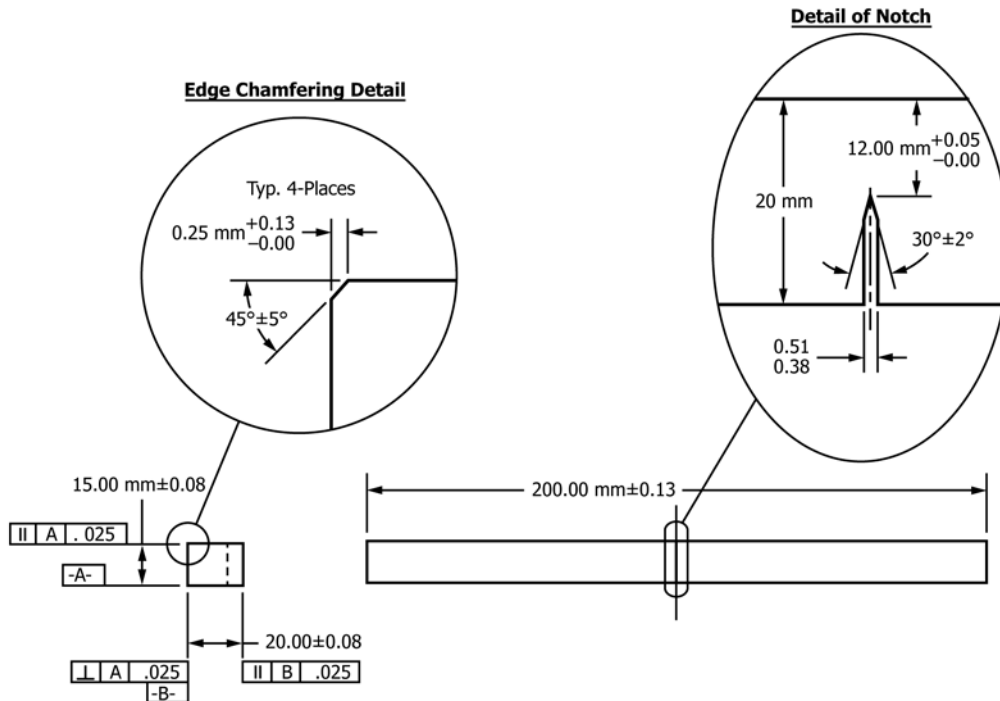
FIG. A1.3 Typical Test Specimen
