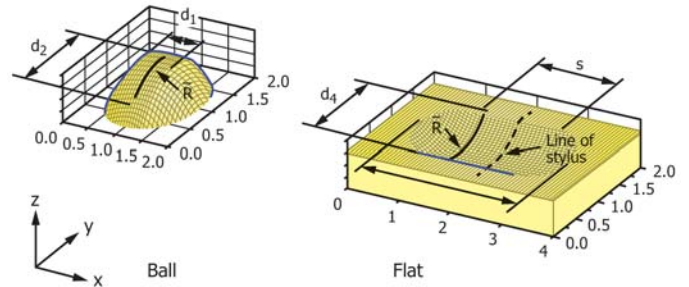
FIG. 4 Scheme of Variables Used to Calculate the Wear Volume of Ball and Disk
