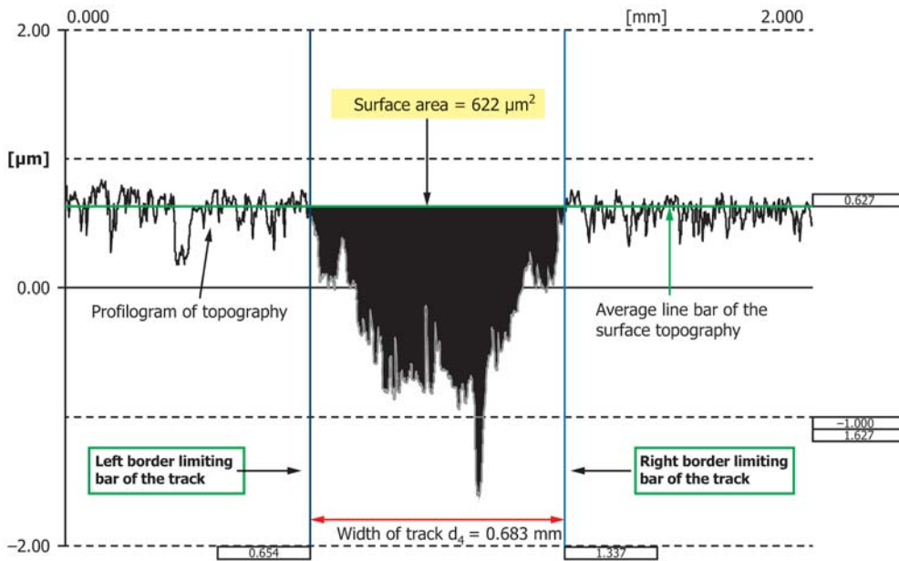
FIG. X1.1 Profilogram Displayed On a Screen and Taken Perpendicular in the Center of the Wear Track on a SRV Test Disk
