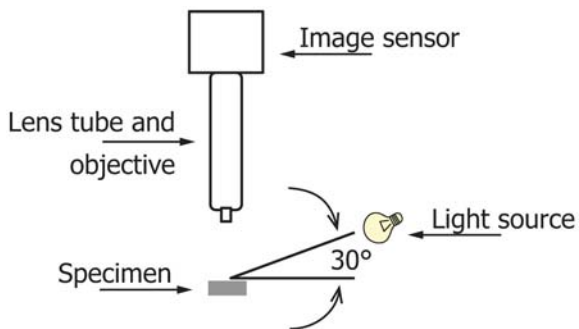
FIG. 3 Darkfield Illumination
