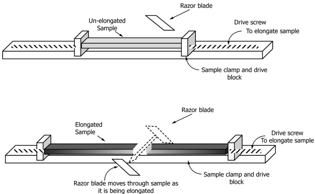
FIG. 2 Bi-Directional Cut
