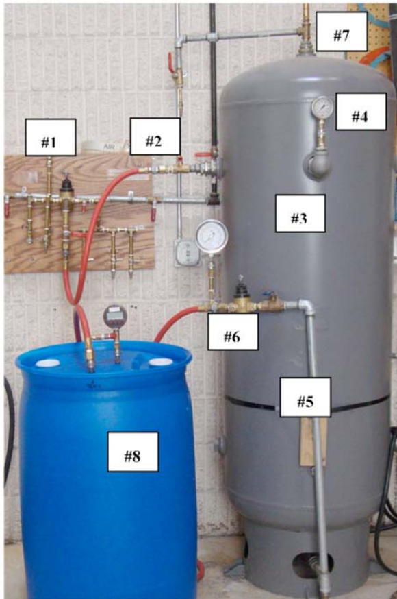
FIG. 2 Larger Container Internal Hydrostatic Pressure Station Example (Photograph)
