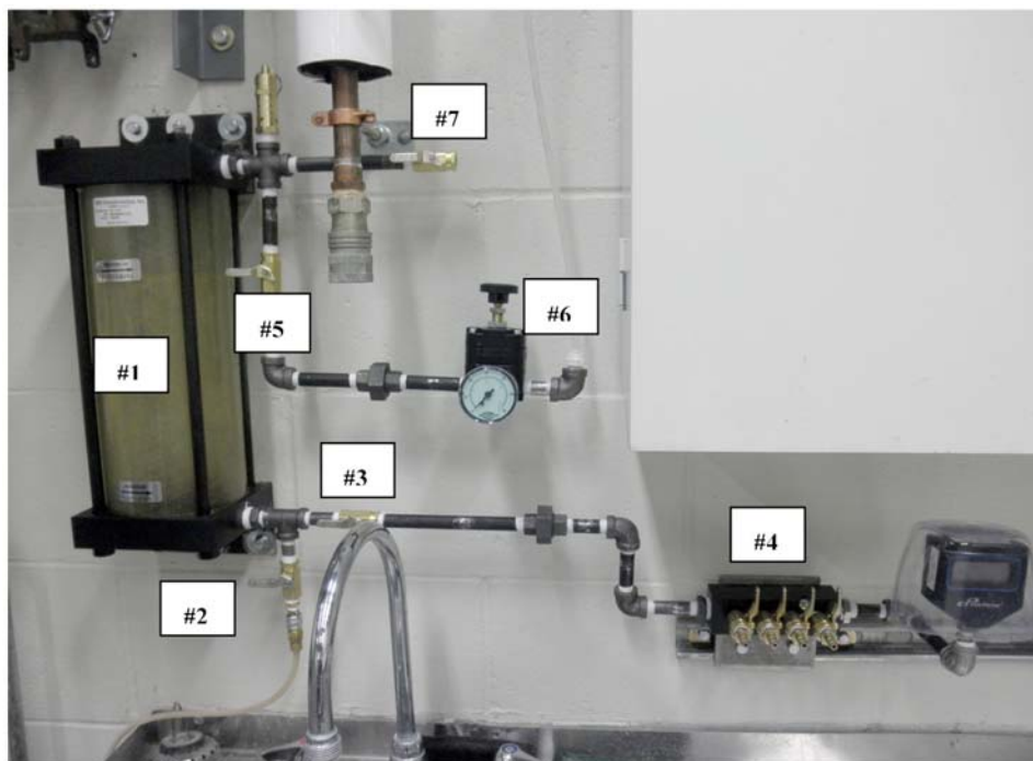
FIG. 3 Small Container Internal Hydrostatic Pressure Station Example
