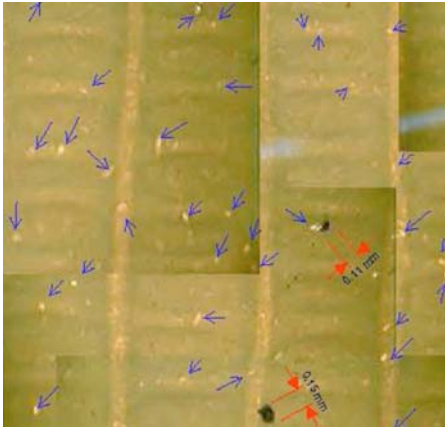
FIG. 8 Many Pinholes Found at Center of Filter
