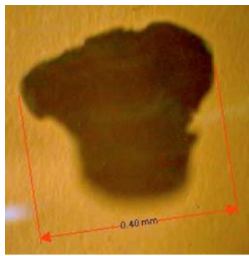
FIG. 3 Particulate Images by Transmission Microscope
