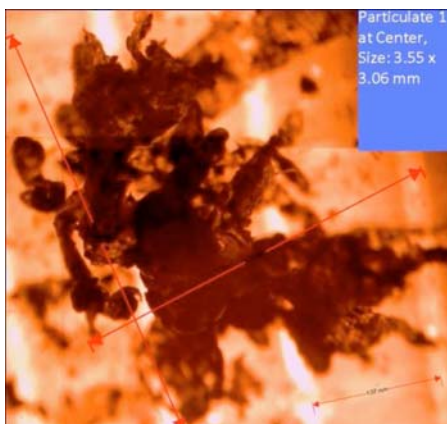
FIG. 7 Overlapped Particulates Found at Center of Filter
