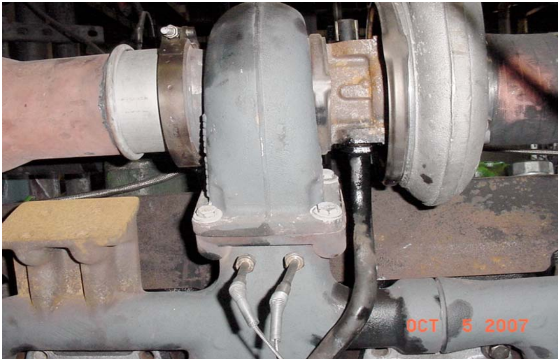
FIG. A4.6 Exhaust Temperature Location
