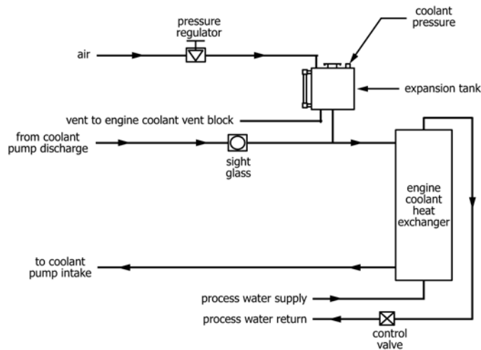
FIG. X1.3 Coolant System (Typical)
