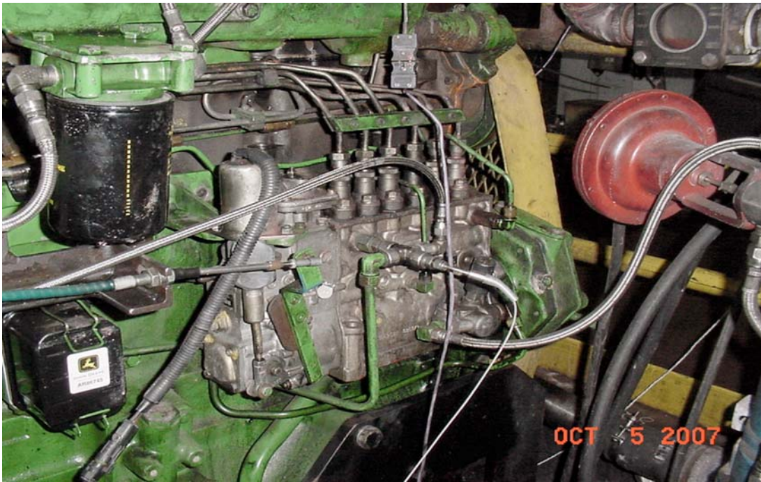
FIG. A4.5 Fuel In Temperature and Pressure Location
