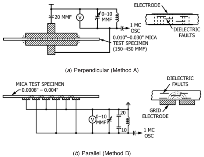
FIG. X1.1 Schematic Arrangement of Test Circuits
