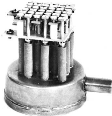
FIG. X1.5 Grid Electrode
