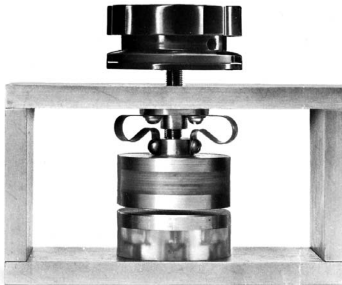
FIG. X1.2 Test Electrodes
