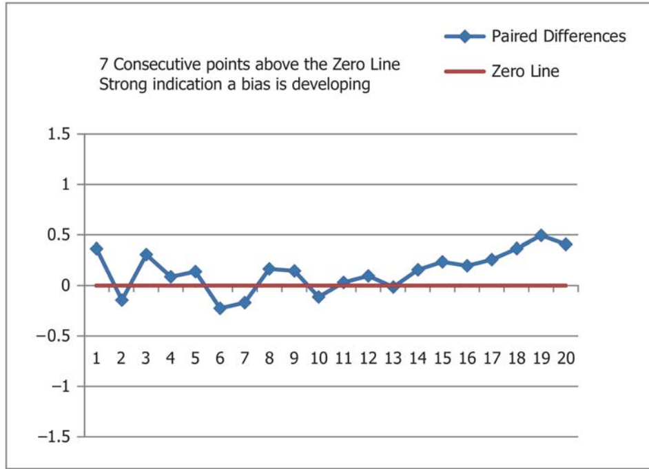
FIG. X3.1 Single Rule Control Chart
