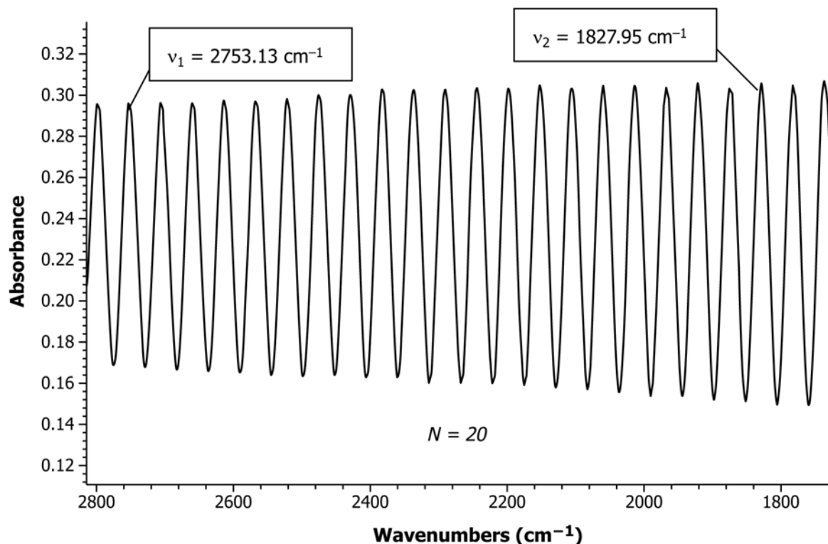
FIG. X2.1 Spectrum of an Empty Cell Used for Calculation of Cell Pathlength
