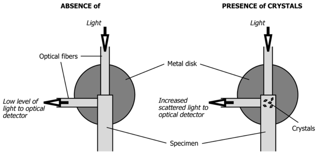
FIG. A1.2 Working Principle (Top View of Key Components)
