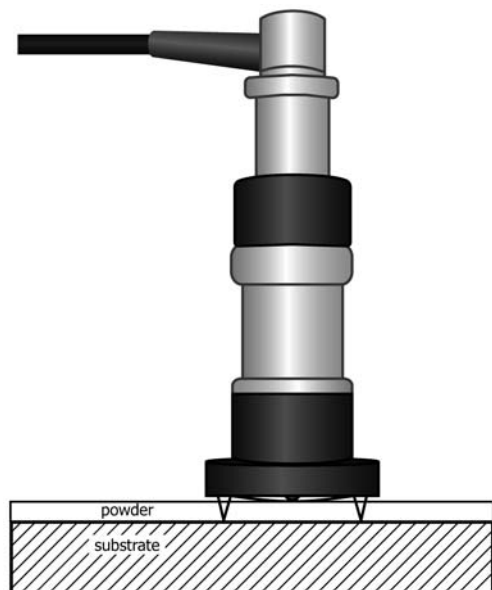
FIG. 3 A Powder Probe
