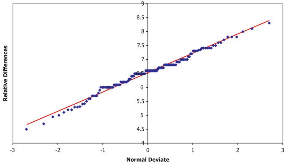
FIG. X3.4 Normal Deviate Plot for Sulfur in #2 Diesel by Test Method D5453
