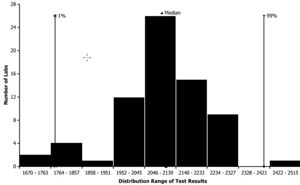
FIG. X3.5 ILCP Histogram for Calcium in Engine Lube Oil by Test Method D5185
