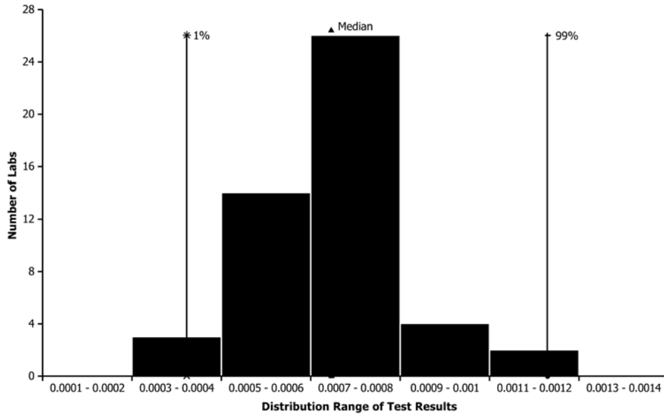
FIG. X3.7 ILCP Histogram for sulfur in #2 Diesel Fuel by Test Method D2622
