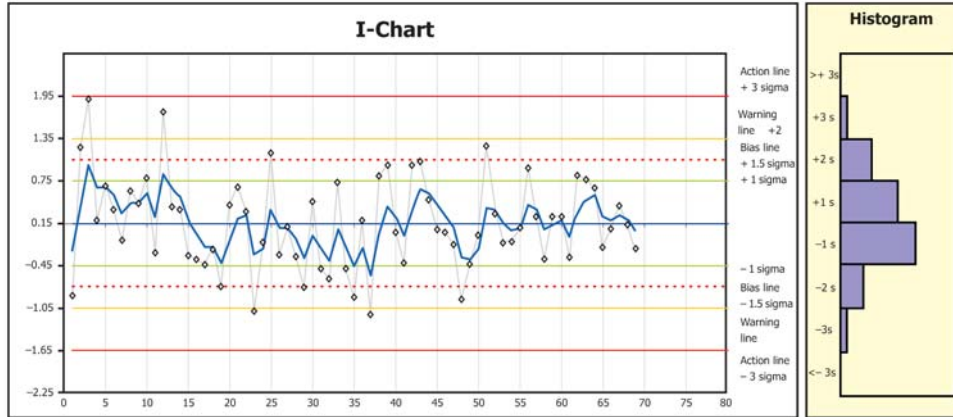
FIG. X3.10 Single Lab Deviations from the Mean, for Sulfur in ULSD by Test Method D5453 Plotted on a Control Chart (I-Chart with EWMA)
