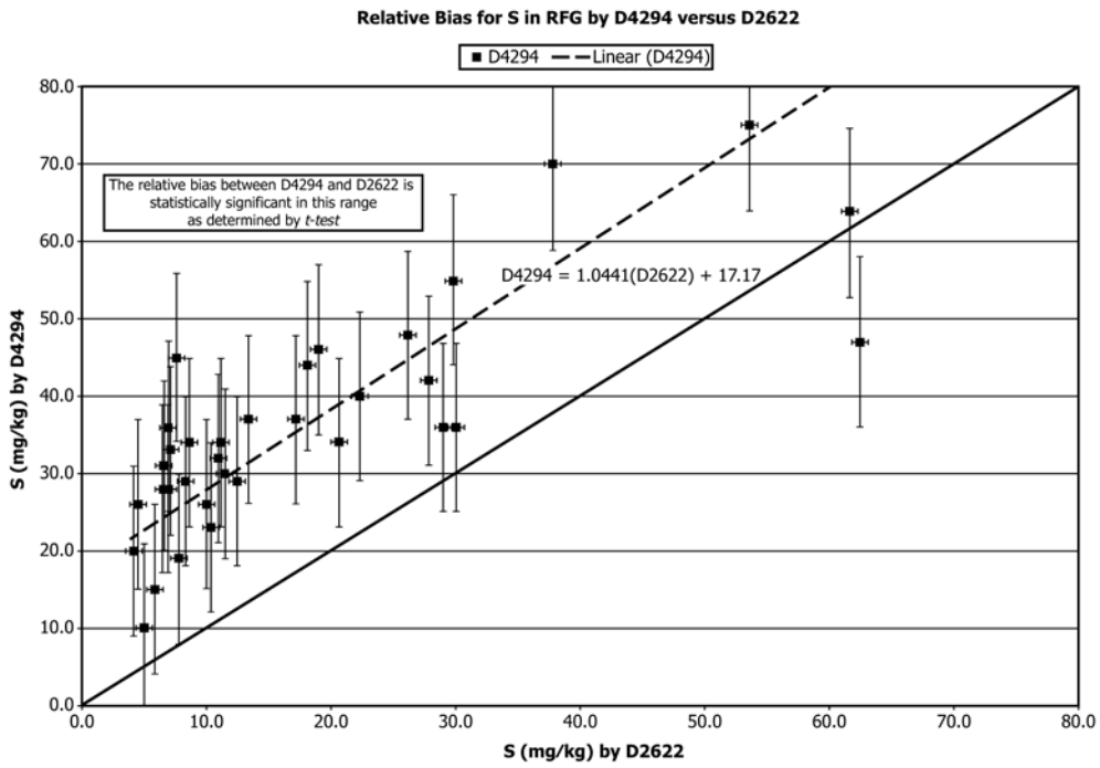
FIG. X3.17 Plot of Mean Sulfur in RFG by Test Method D4294 versus D2622 ; Each Data Point Represents a Program Cycle
