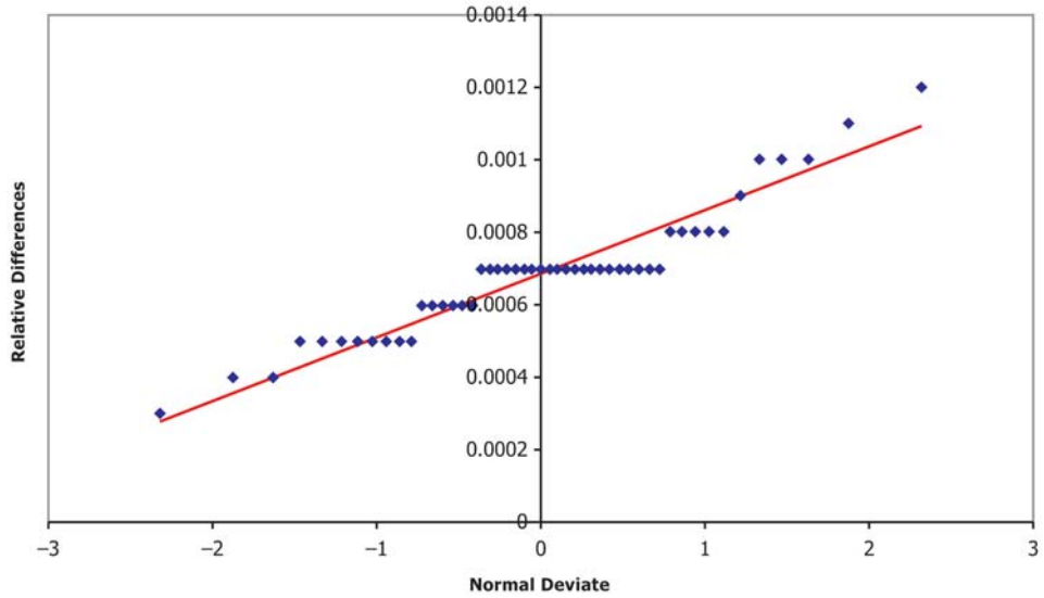
FIG. X3.8 Normal Deviate Plot for Sulfur in #2 Diesel by Test Method D2622
