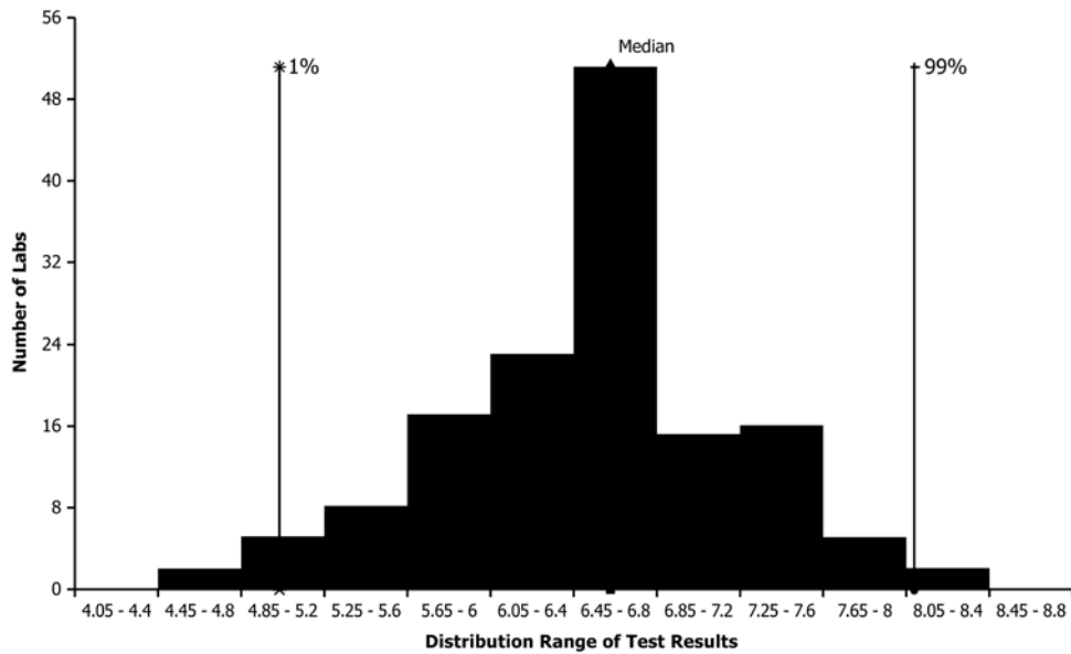
FIG. X3.3 ILCP Histogram for Sulfur in #2 Diesel by Test Method D5453
