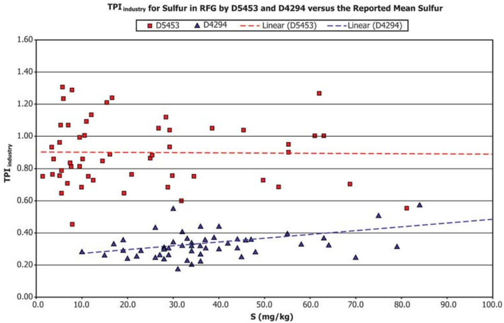
FIG. X3.21 TPI (Industry) for Sulfur in RFG by Method versus Mean Sulfur
