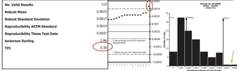
FIG. X3.14 Combined Use of the ILCP Result Table, Statistical Summary, and Graphs to Identify Opportunities for Improvement
