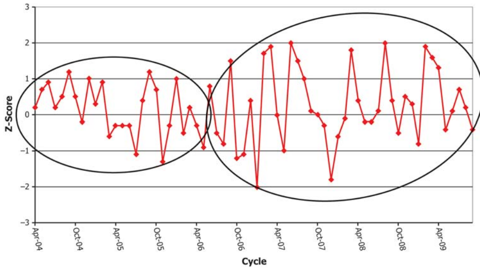
FIG. X3.12 Plot of Z-Scores for Single Lab for Sulfur in ULSD by Test Method D5453 Covering Multi-year Period
