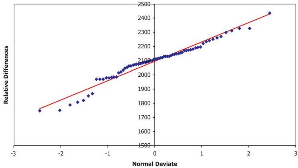
FIG. X3.6 Normal Deviate Plot for Calcium in Engine Lube Oil by Test Method D5185
