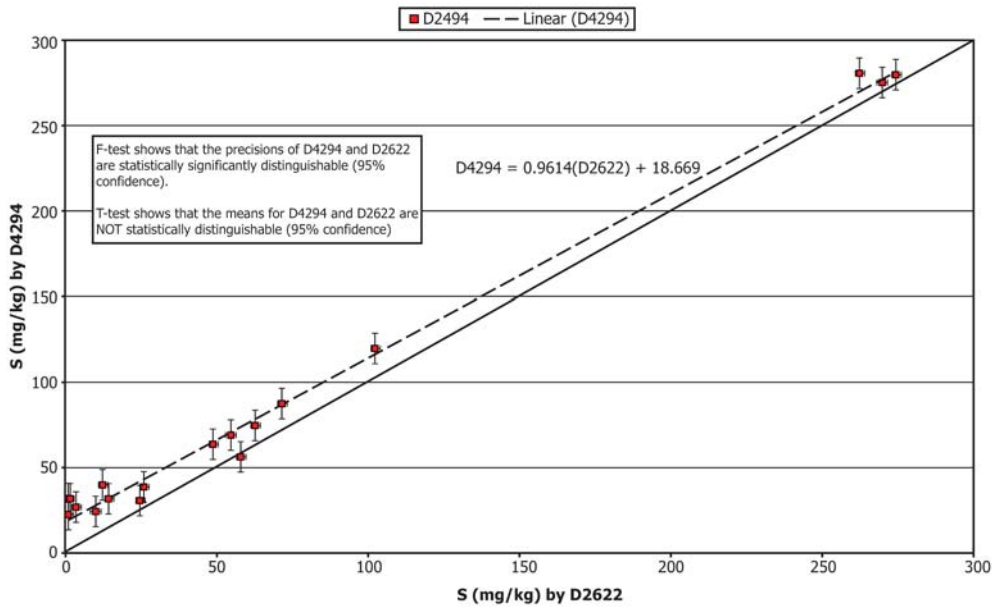
FIG. X3.19 Mean Sulfur in Mogas by Test Method D5453 versus D2622 Covering Numerous ILCP Cycles
