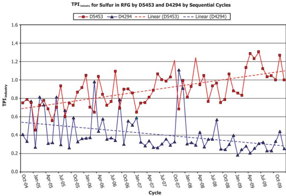
FIG. X3.20 TPI (Industry) for Sulfur in RFG by Test Method D5453 and D4294 by Proficiency Test Cycle
