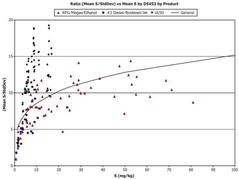
FIG. X3.25 Ratio of Mean to Standard Deviation versus Mean Sulfur by Test Method D5453 by Product
