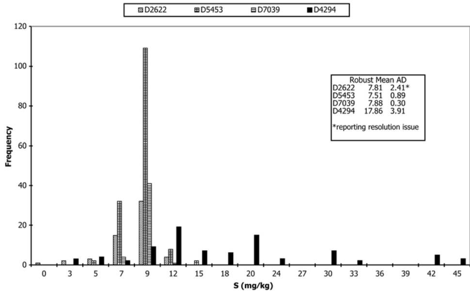
FIG. X3.9 Distribution of Sulfur Results in an ILCP #2 Diesel Fuel Sample by Four Test Methods
