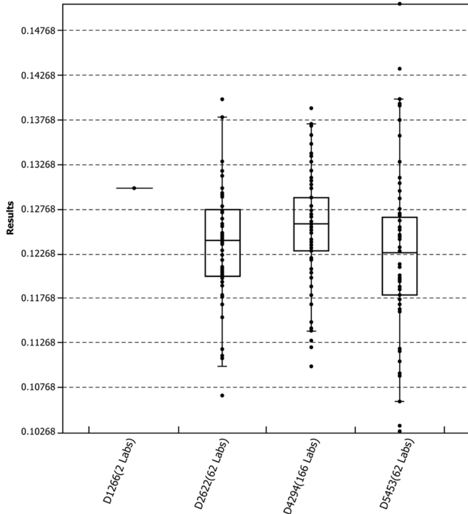
FIG. X3.15 Box and Whisker Plots for Sulfur in Jet Fuel (03/2009 Cycle); Test Methods D1266 (2 Labs), D2622 (62 Labs), D4294 (166 Labs), and D5453 (62 Labs)
