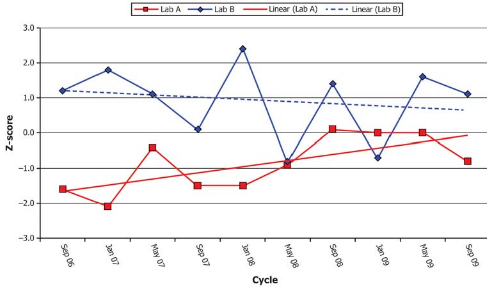
FIG. X3.13 Historic Z-scores for Calcium in Lube Oil by Test Method D4951; PI = 1.07 and 0.79 for Labs A and B, Respectively
