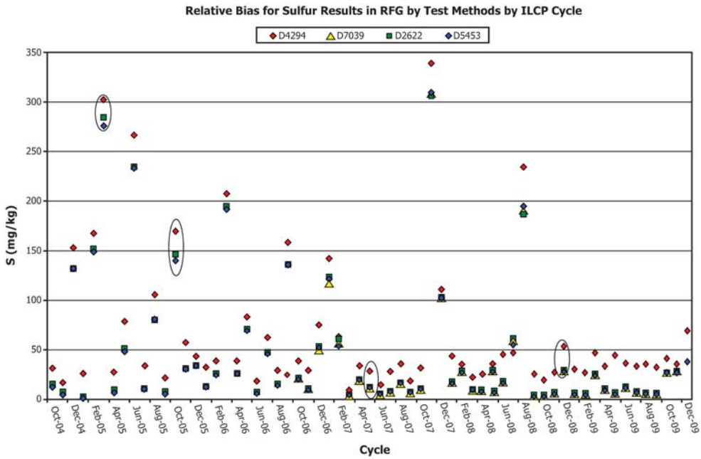
FIG. X3.16 Plot of Means by Test Methods by ILCP Cycle for Sulfur in RFG
