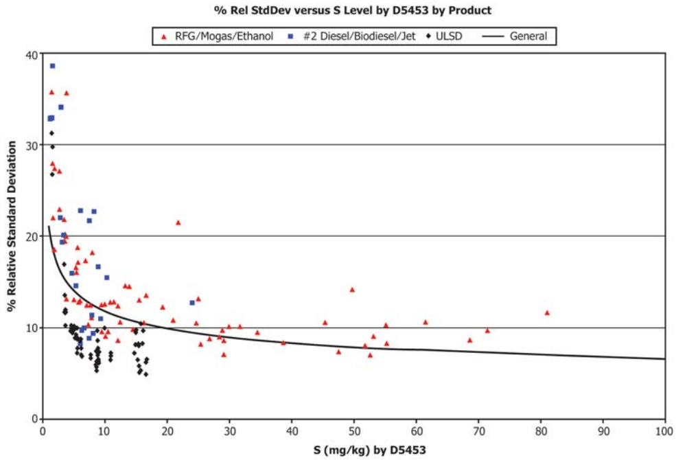
FIG. X3.24 Percent Relative Standard Deviation for Mean Sulfur by Test Method D5453 by PT Product
