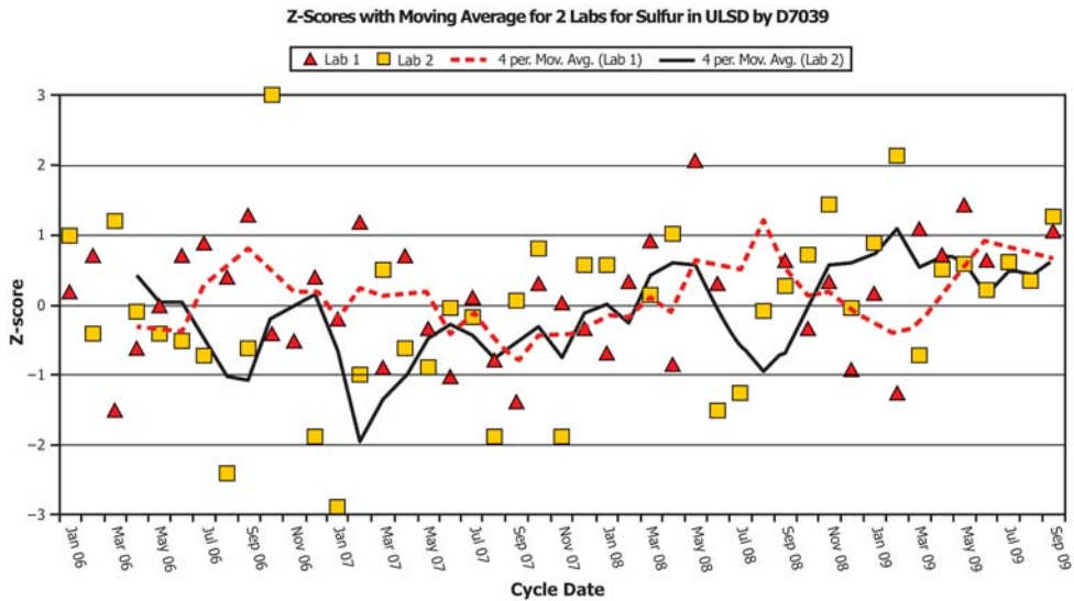
FIG. X3.11 Z-scores (with Moving Average) for Determination of Sulfur in ULSD by Test Method D7039; Plotted Sequentially by Sample Date
