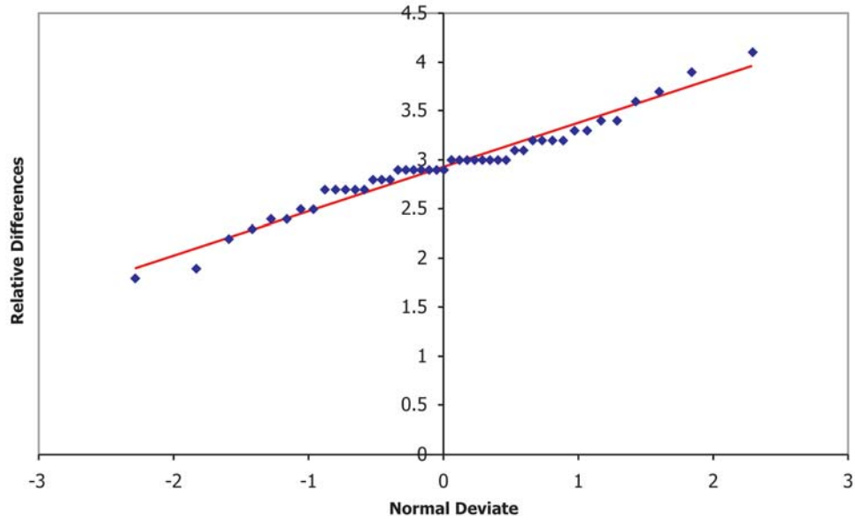
FIG. X3.2 Normal Deviate Plot for Sulfur in #2 Diesel by Test Method D7039
