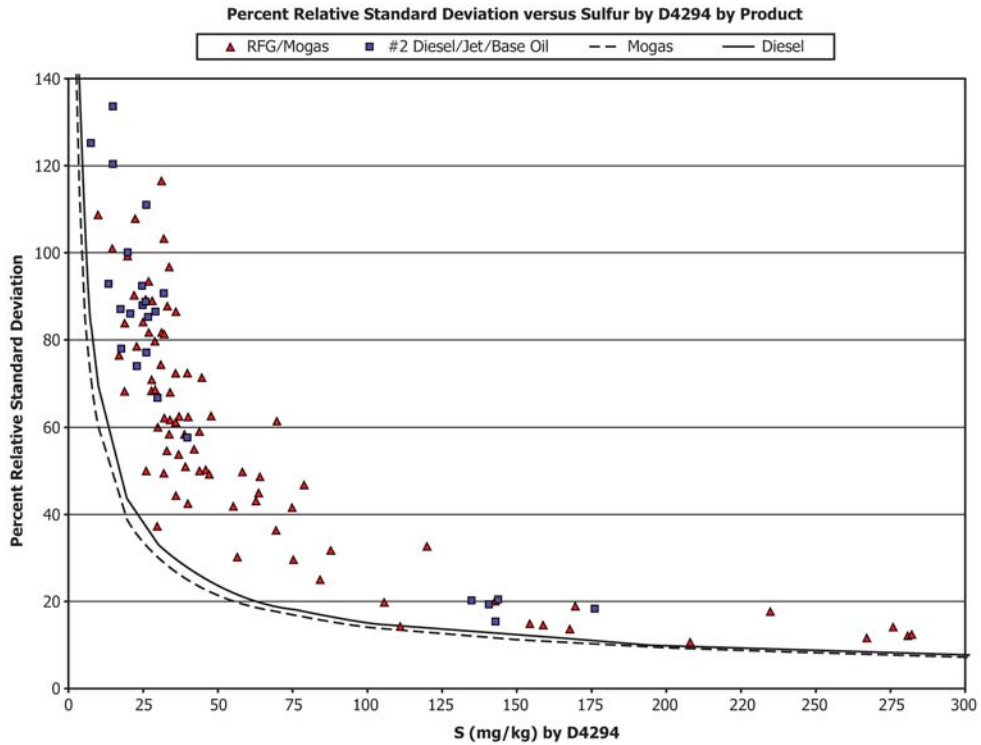
FIG. X3.23 Percent Relative Standard Deviation for Sulfur by Test Method D4294 by PT Product
