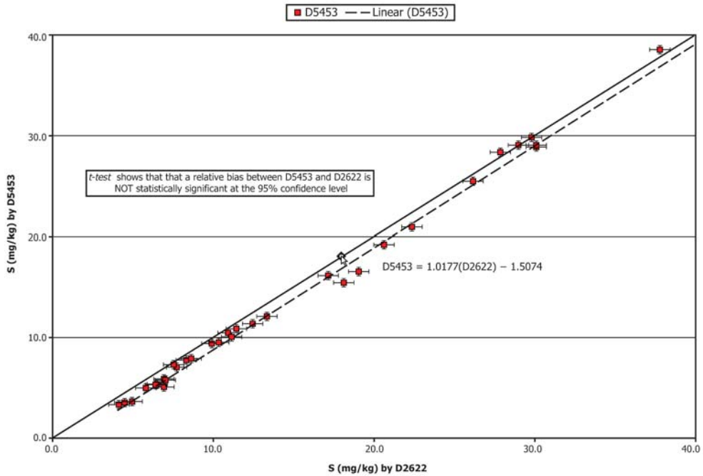
FIG. X3.18 Plot of Mean Sulfur in RFG by Test Method D5453 versus D2622
