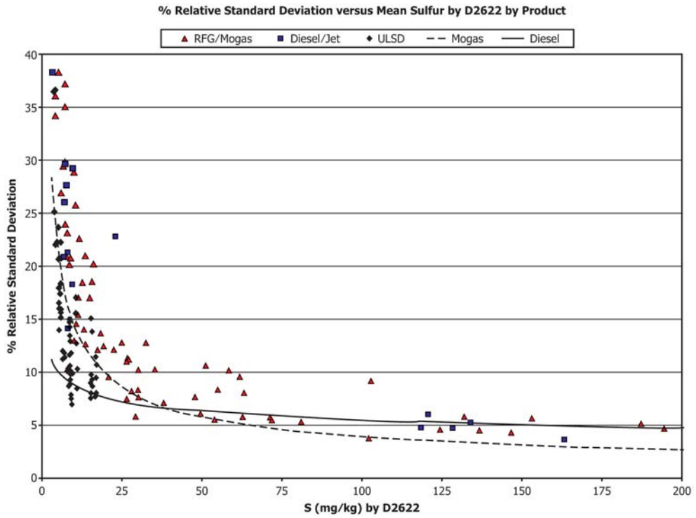
FIG. X3.22 Percent Relative Standard Deviation for Mean Sulfur by Test Method D2622 by PT Product
