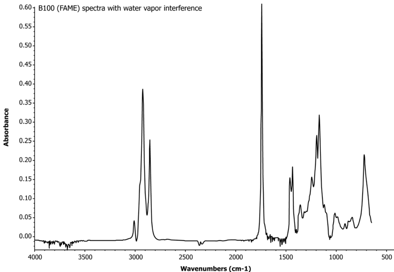
FIG. A3.3 Spectra of B100 (FAME) with Excessive Water Vapor Interference (Full Region)
