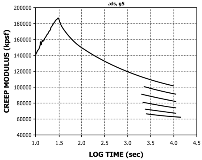
FIG. X1.4 Compressive Creep Modulus vs. Log Time After Rescaling
