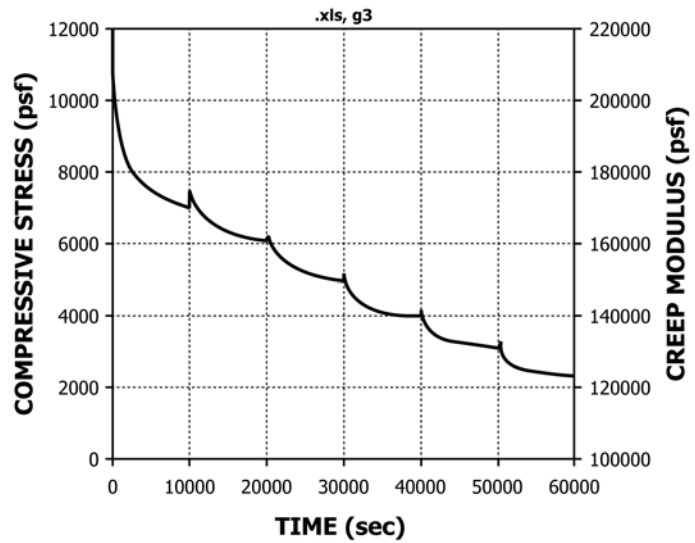
FIG. X1.3 Stress and Compressive Creep Modulus vs. Linear Time
