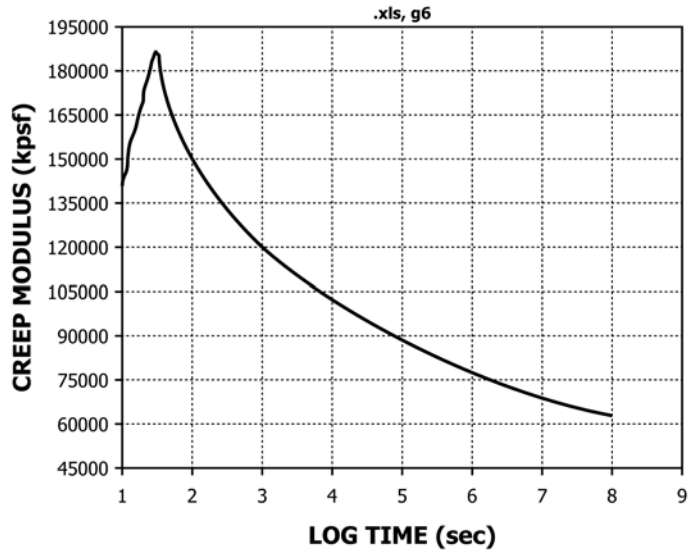
FIG. X1.5 Master Compressive Creep Modulus vs. Log Time Curve at the Step One Reference Temperature
