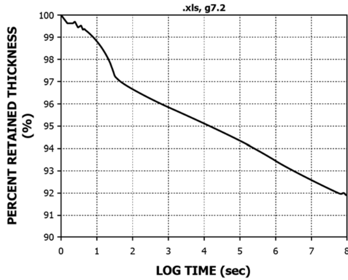
FIG. X1.7 Master Compressive Creep Strain (Plotted as Percent Retained of Original Thickness) vs. Log Time at the Step One Reference Temperature
