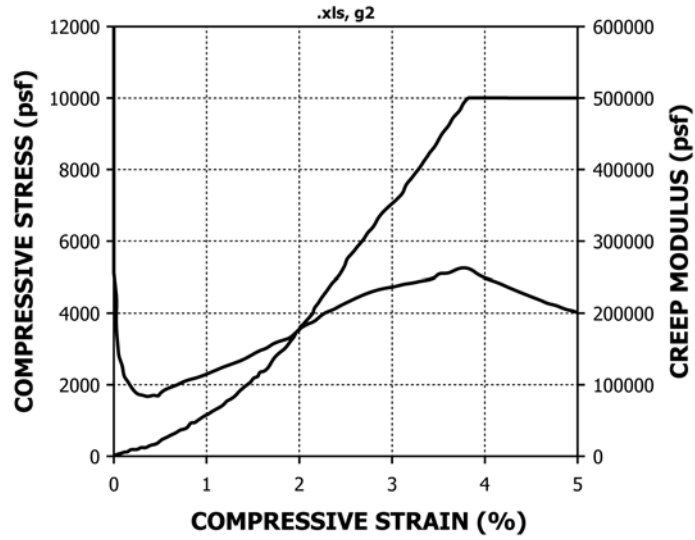
FIG. X1.2 Stress and Secant Modulus vs. Compressive Strain
