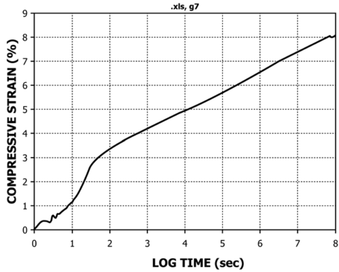
FIG. X1.6 Master Compressive Creep Strain vs. Log Time at the Step One Reference Temperature
