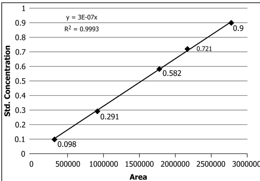
FIG. 13 Typical Olefin Calibration Curve
