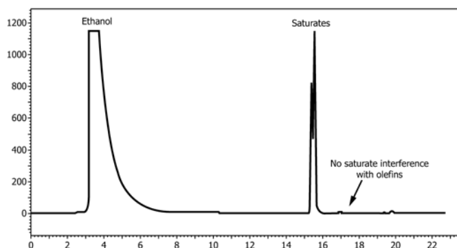
NOTE 1—Loading time mixture D was injected to monitor t_O (9.2.6). FIG. 10 Typical Chromatogram Obtained for Final Method Adjustments
