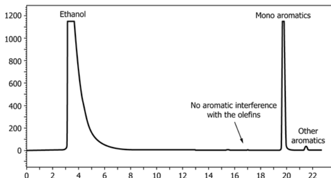
NOTE 1—Loading time mixture E was injected to monitor t_O (9.2.6). FIG. 11 Typical Chromatogram Obtained for Final Method Adjustments
