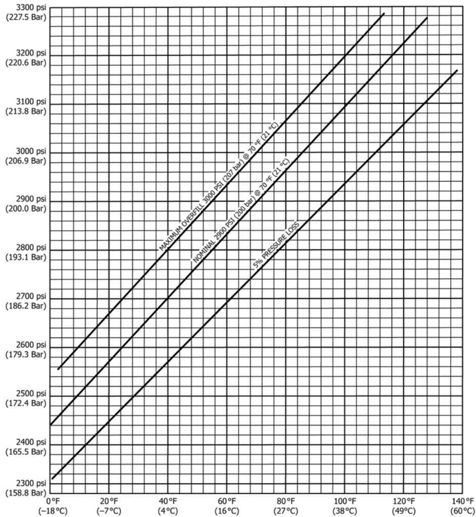
FIG. 2 IG-541 (200 Bar) Isometric Diagram
