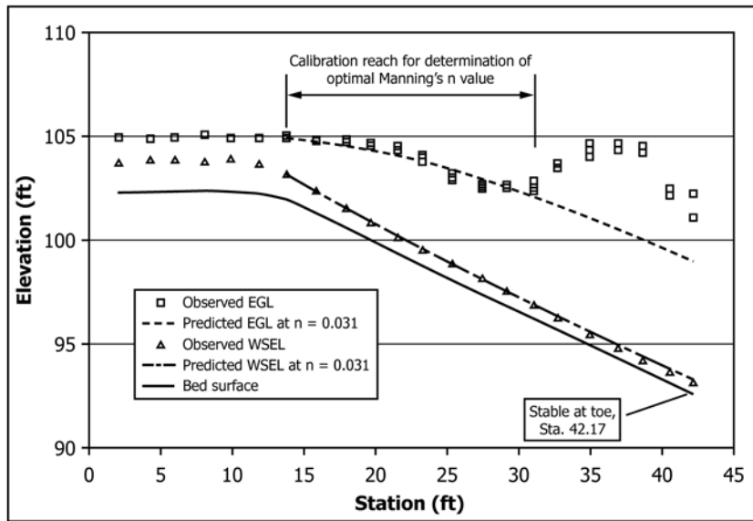
FIG. X1.3 Observed and Predicted Water and Energy Surfaces
