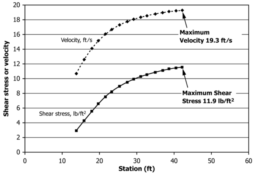
FIG. X1.4 Velocity and Shear Stress Predicted by Step-Forewater Analysis
