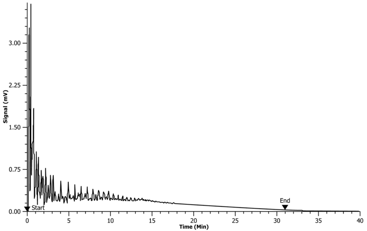
FIG. A1.4 Chromatogram (Baseline Corrected) of a Crude Oil (Injected at -20 °C)
