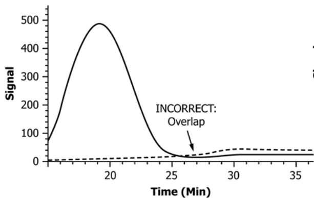
FIG. A1.6 Correct and Incorrect Relative Position of Baseline and Sample Signal
