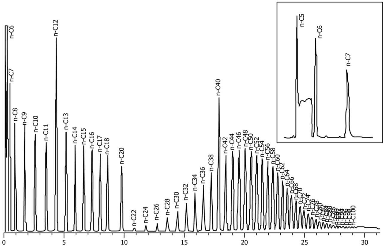
FIG. A1.2 Chromatogram of the Retention Time Calibration Mixture C 5 -C 100 Injected at -20 °C, Insert Expands View of C 5 -C 7 Region
