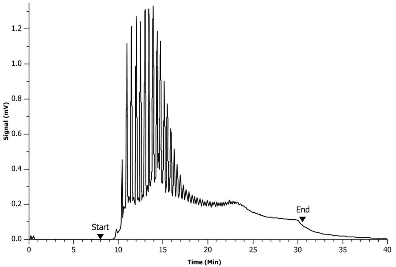
FIG. A1.5 Chromatogram (Baseline Corrected) of an Atmospheric Residue
