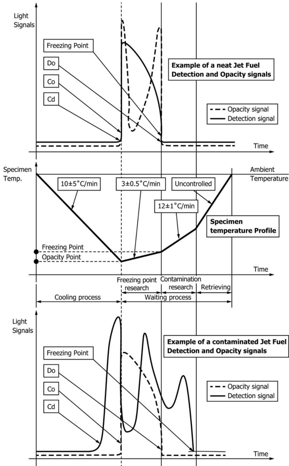
FIG. A1.5 Testing Process Chart
