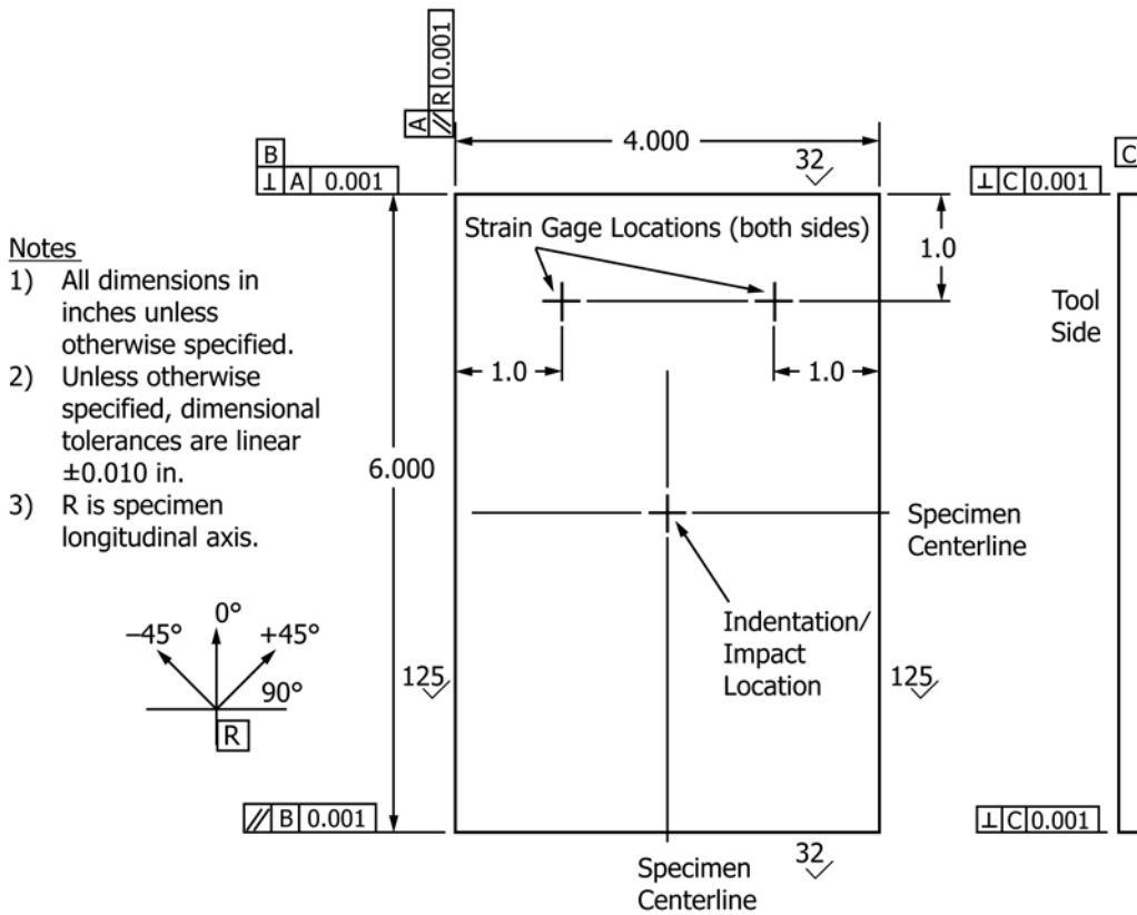
FIG. 11 Compressive Residual Strength Test Specimen (Inch-Pound Version)
