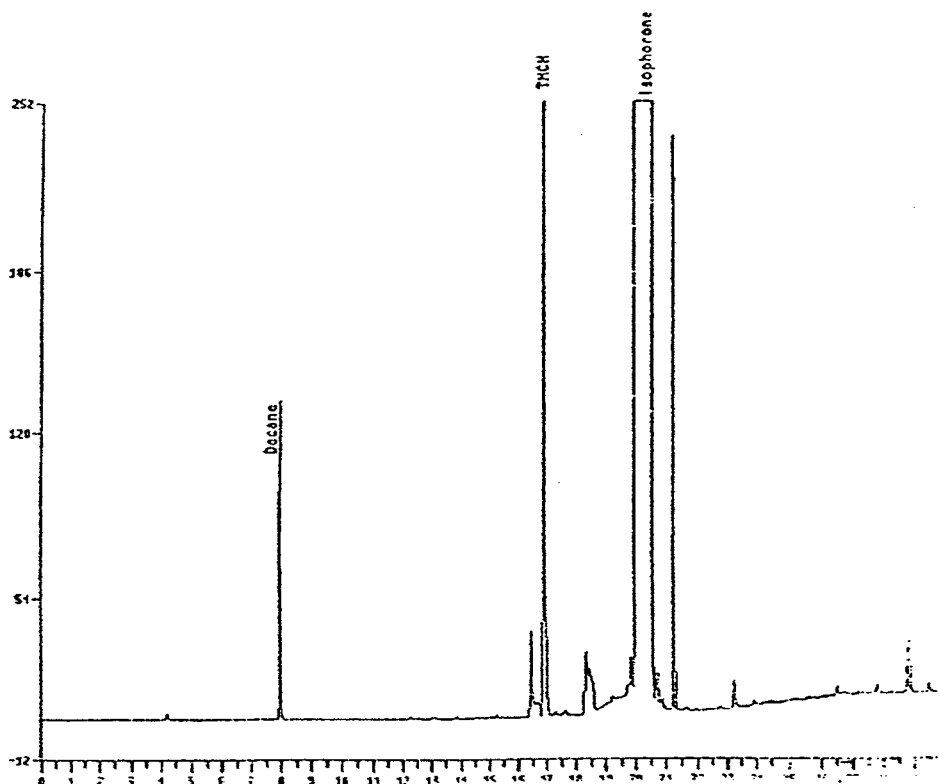
FIG. 1 Typical Isophorone Chromatogram
