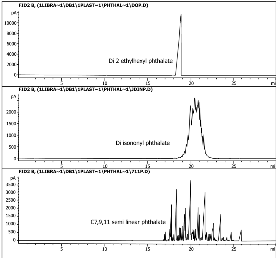
FIG. 1 Chromatogram Example
