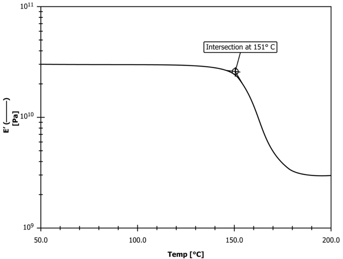
FIG. X1.3 An Example of the Intersection Drawn Where the First Tangent Line is Selected Too Close to the Transition and the Second Tangent Line is Selected Too Close to the Transition for the DMA Tg value.
