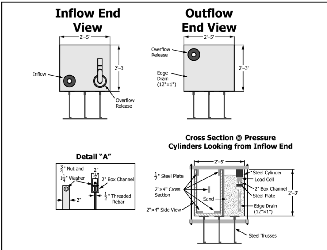
FIG. X1.3 Inflow and Outflow End Views
