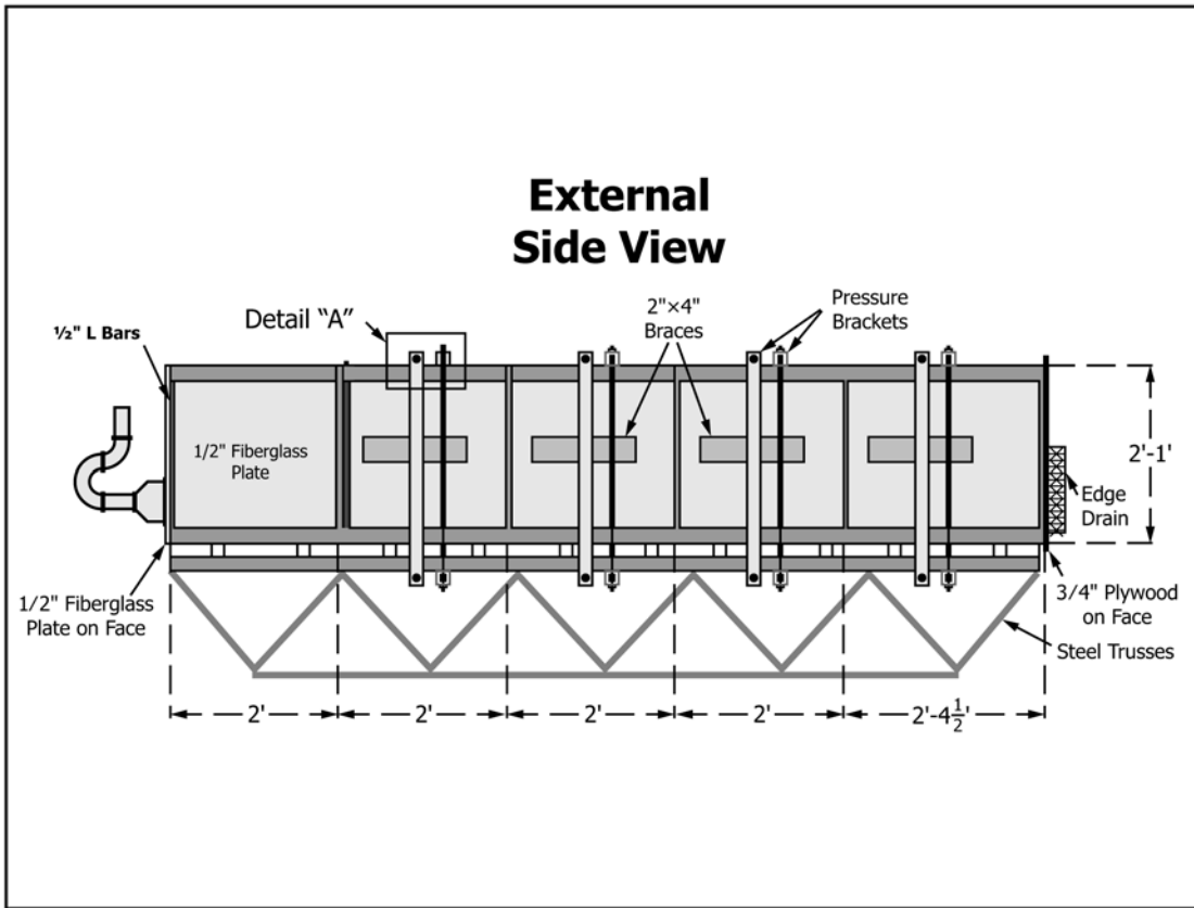
FIG. X1.1 External Side View
