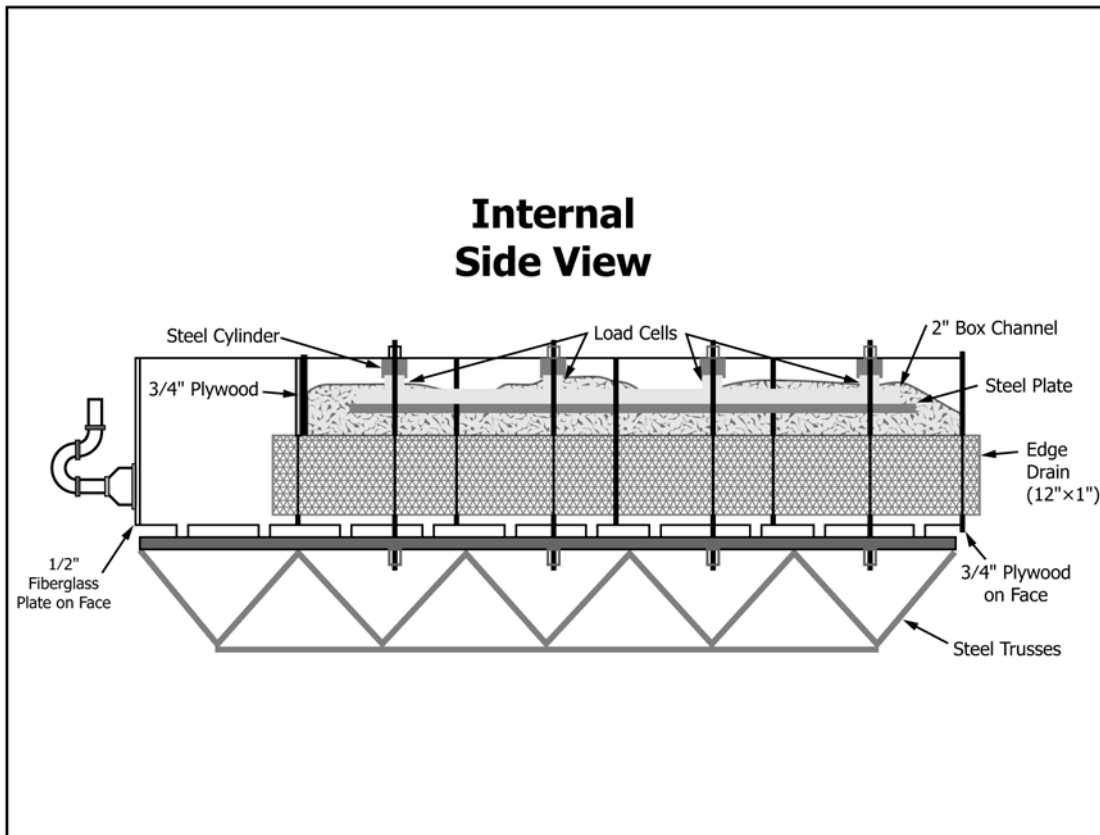
FIG. X1.2 Internal Side View
