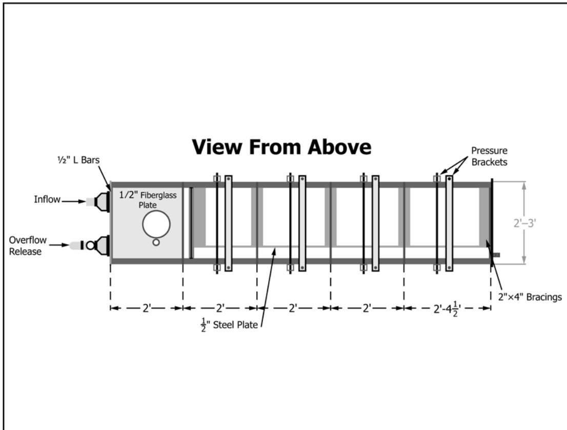
FIG. X1.4 View from Above
