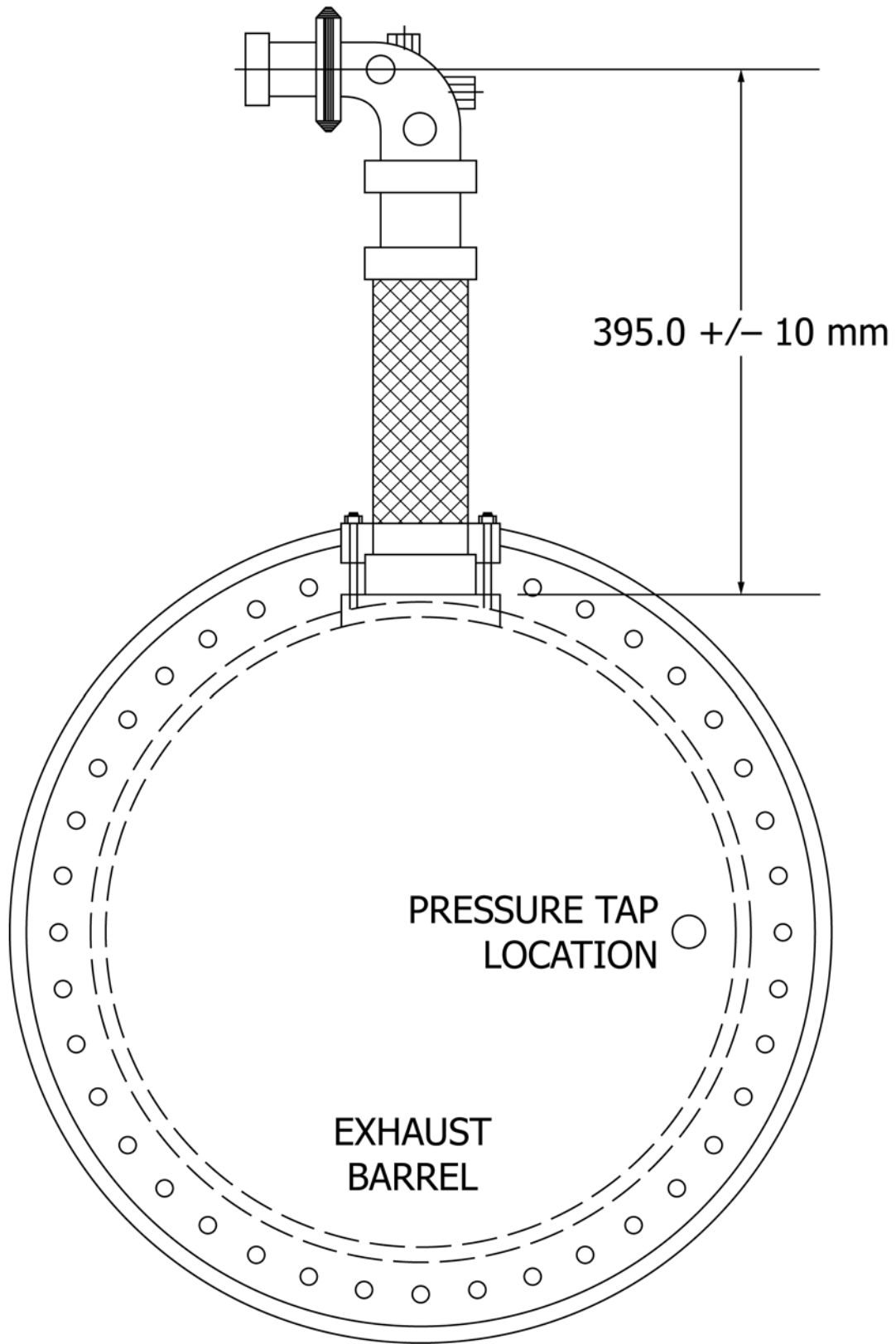
NOTE 1—1Y3789 Exhaust Connector Group Arrangement. See parts book for individual parts. FIG. A2.7 1Y3978 Exhaust Barrel Piping and Pressure Locations
