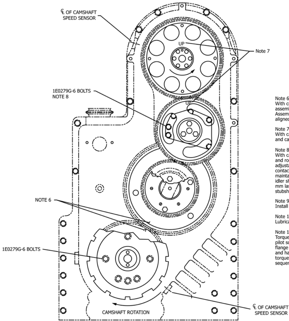
FIG. A8.6 1Y3700 Engine Timing
