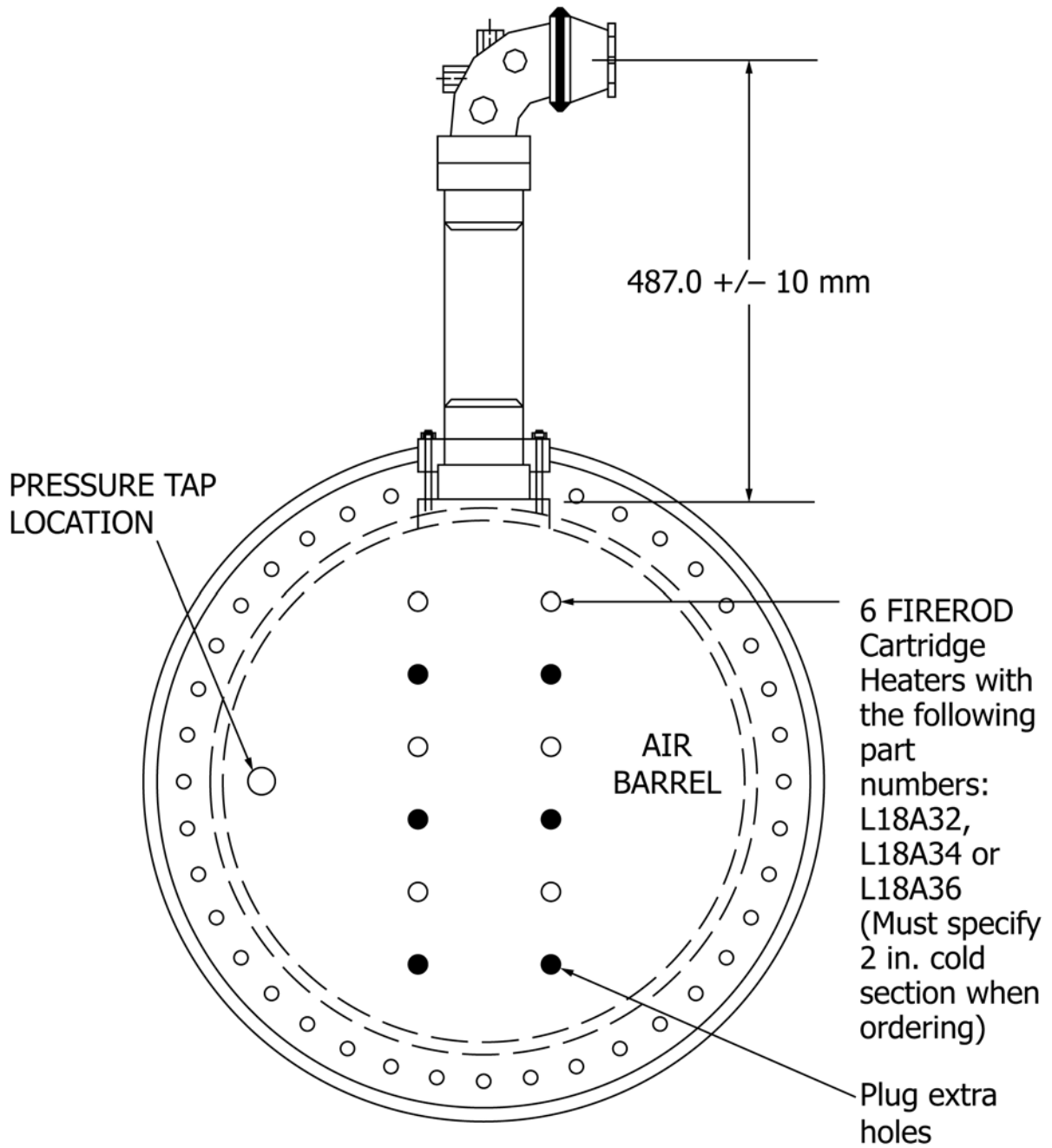
FIG. A2.8 1Y3976 Intake Air Barrel Piping and Pressure Locations
