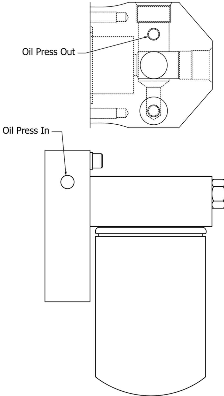
FIG. A2.6 Oil Filter Delta Pressure Locations—Right Side View
