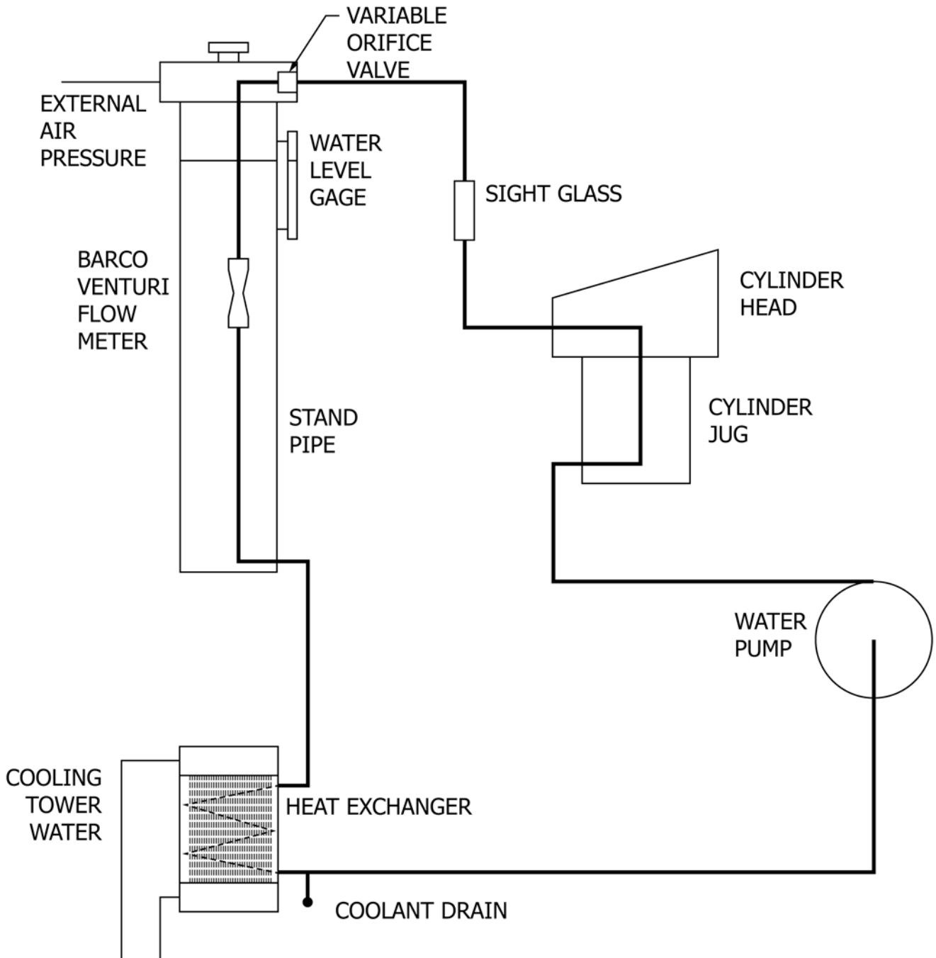
NOTE 1—See Table A3.1 for sight glass details. FIG. A3.1 Engine Cooling System Arrangement
