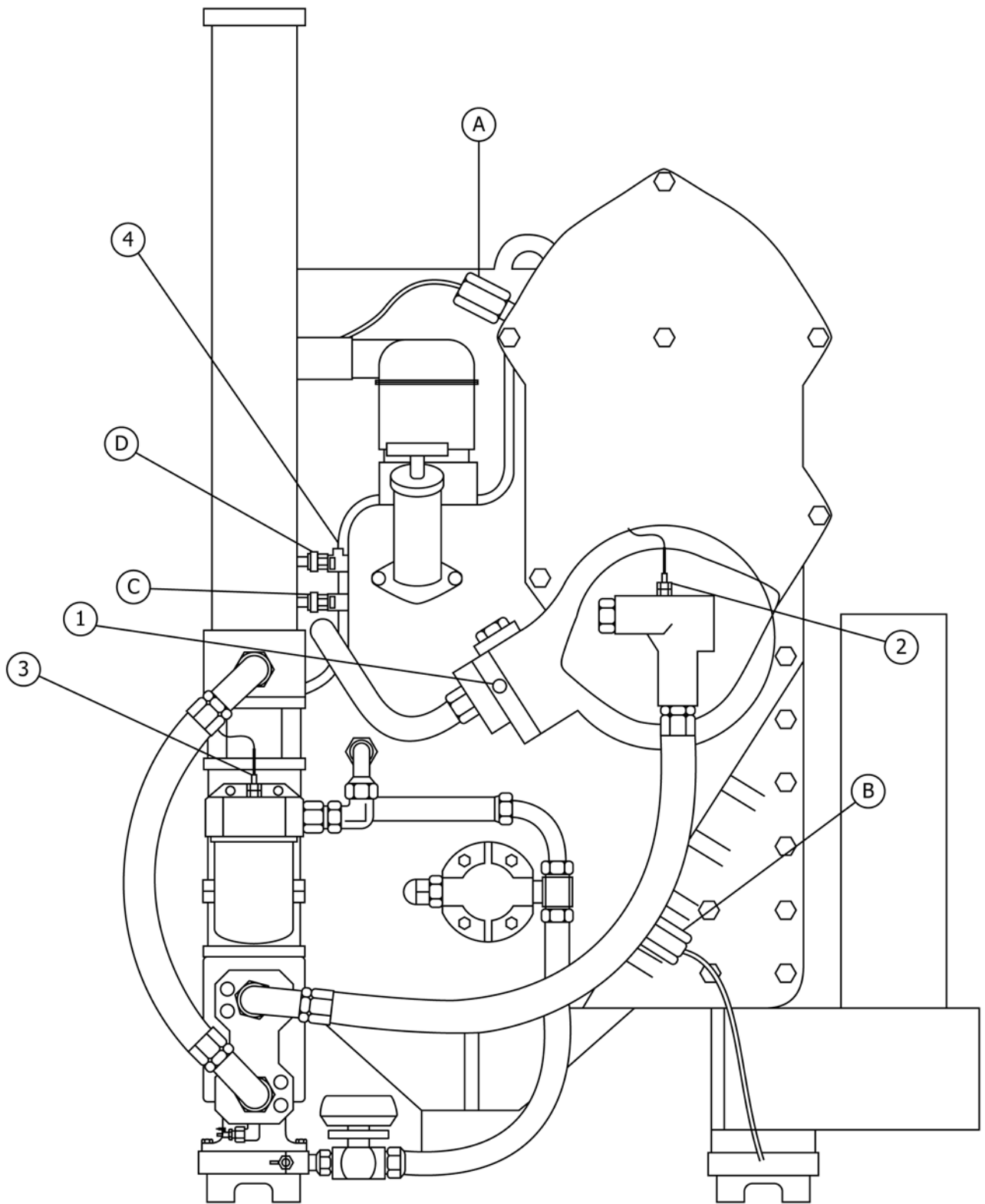
FIG. A2.1 Instrument Locations—Engine Front View
