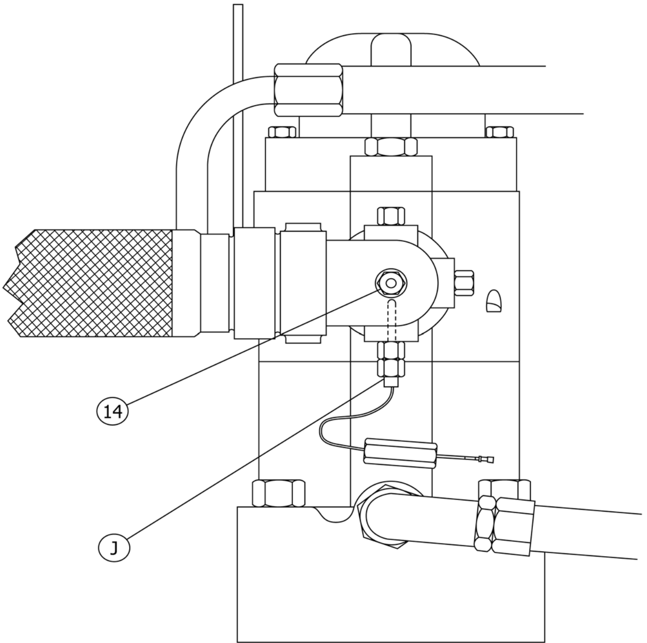
FIG. A2.3 Instrument Locations—Right Engine View
