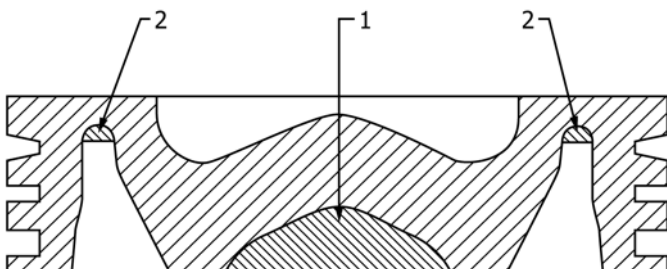
Area (1)—Under-crown: All surfaces of the under-crown including transition radius, but not the vertical sides of the pin bore struts.
