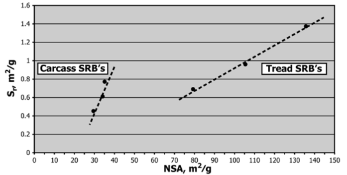
FIG. A1.1 SRB-6 Series STSA Repeatability Standard Deviation
