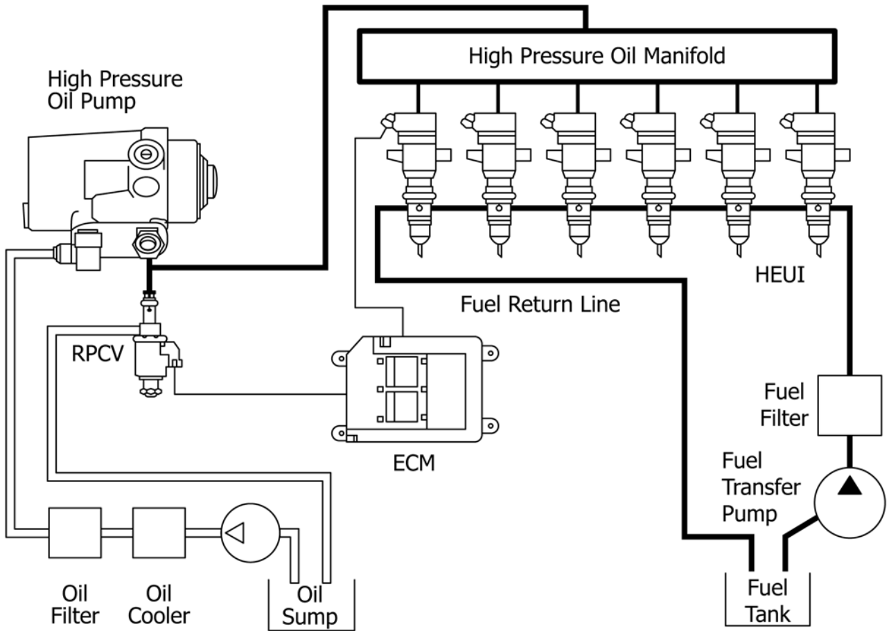
FIG. A1.1 HEUI System Components
