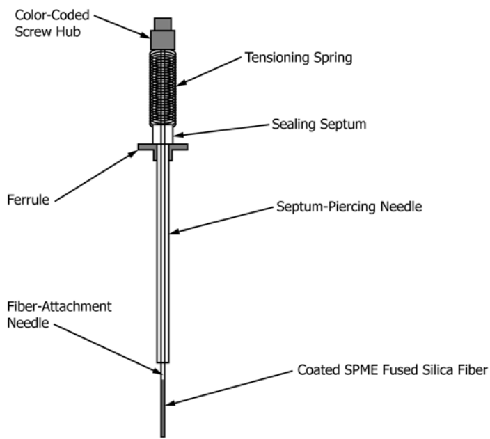
FIG. 1 Fiber Holder
