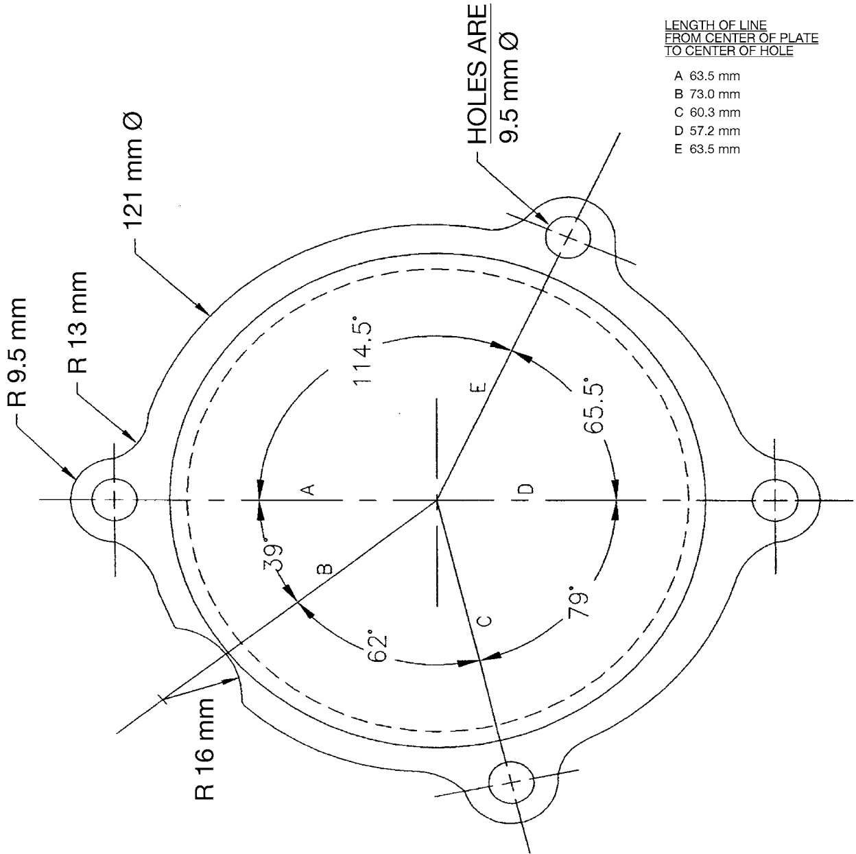
FIG. A2.6 Water Pump Plate
