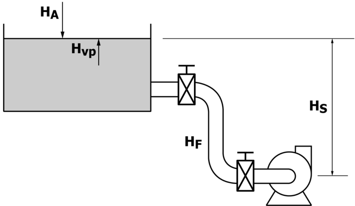
FIG. 5 Illustration of NPSH Parameters
