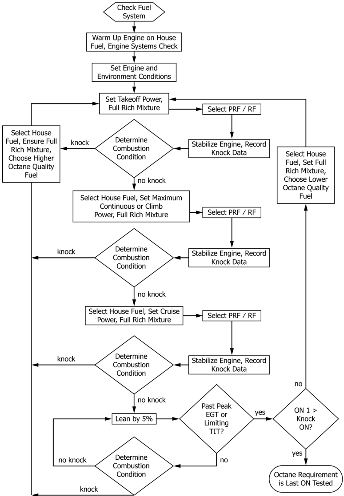
FIG. 1 Flow Chart Illustrating the Octane Rating Procedures
